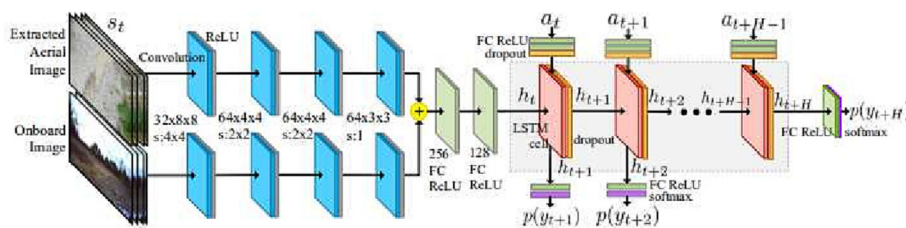
Fig. 15. The proposed learning-based setup of Manderson et al. model to categorize terrain types [83].
