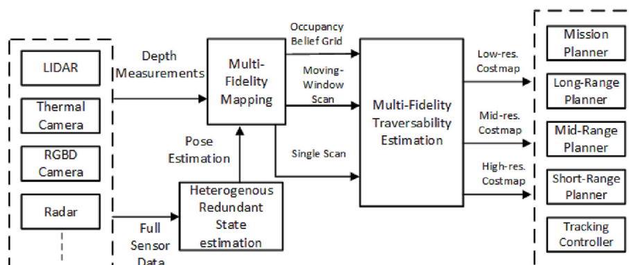
Fig. 10. Overall Layout of Resilient Multi-Fidelity (RMF) Method [142].
