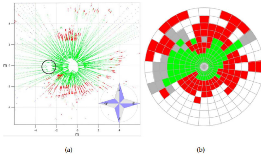
Fig. 4. Top View of 3D Point Cloud (a), Traversability Map (b) [84].
