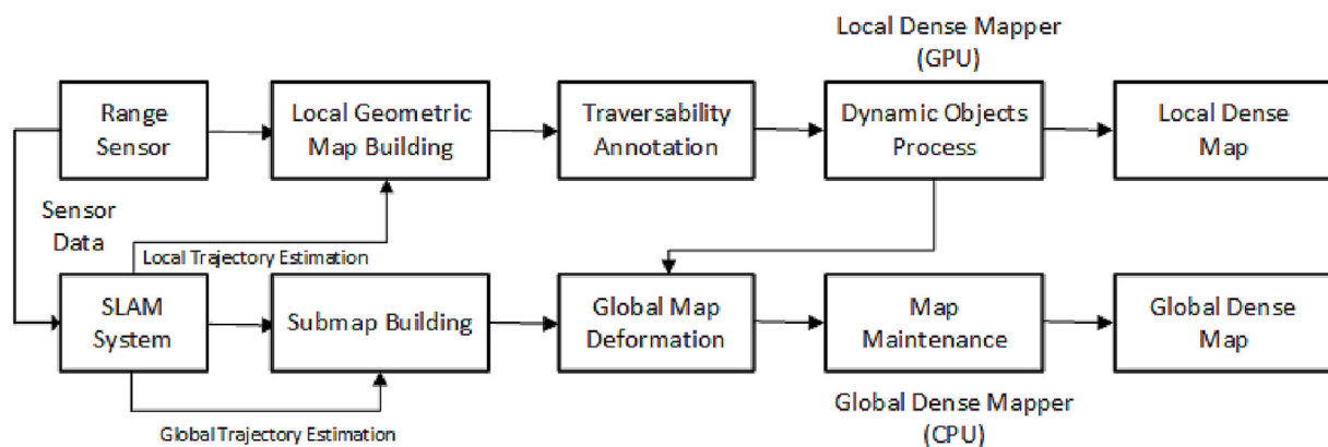
Fig. 9. Overview of the Proposed GEM Algorithm [103].
