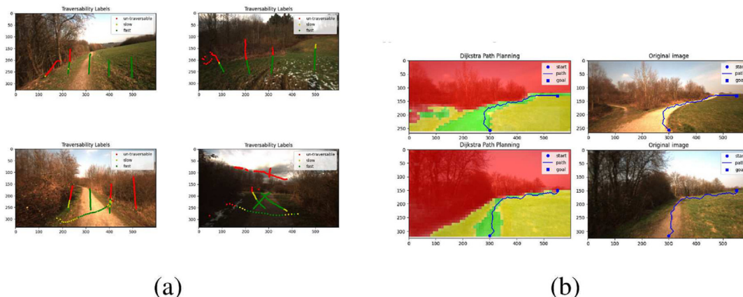
Fig. 14. Kester-et-al: (a) Labelled Images snapshot, (b) Path Planning Algorithm results [15].
