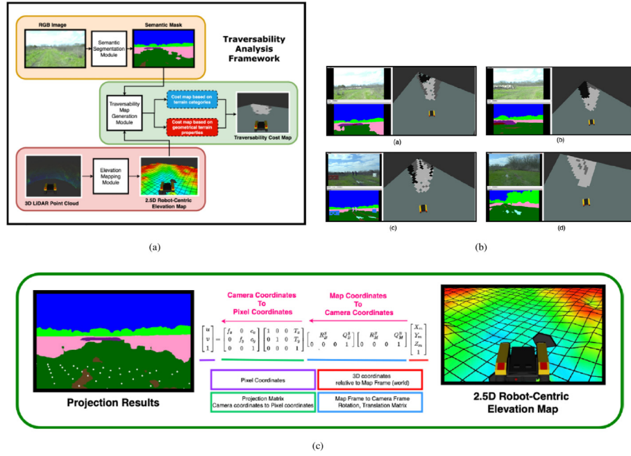
Fig. 11. Figure info: (a) the main framework, (b) Visualization of Traversability Cost Map (in each image the top-left is the main image, bottom-left is the semantic mask, and on the right is the terrain traversability cos map. Darker colour shade represents the less traversable area, (c) the Projection Process [79].
