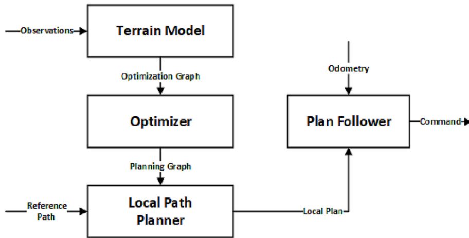
Fig. 7. The Schematic Diagram of the Optimization-based Terrain Modelling and Path Planning in Graf et al.[41].
