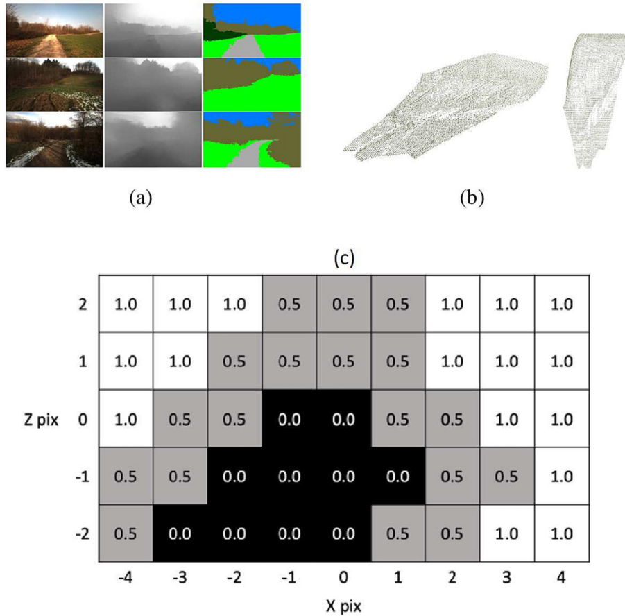
Fig. 12. Broatch-et-al: (a) Freiburg Forest Dataset snapshot, (b) Terrain point cloud, (c) Pixel Position and Depth Values [15].
