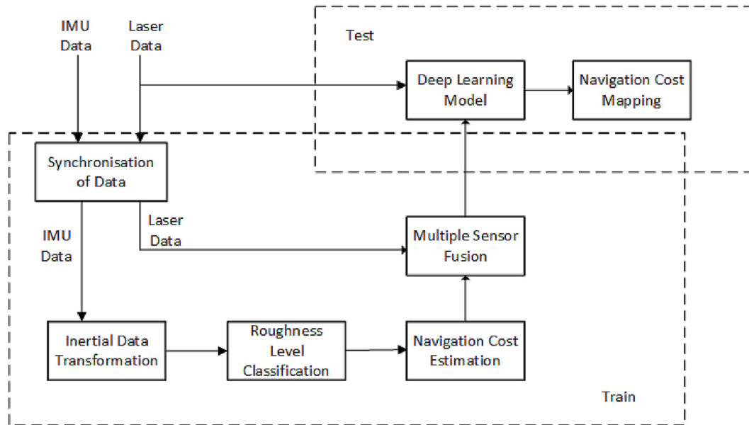
Fig. 8. The Overall Layout of the Three-Dimensional Mapping Method by Oliveira et al. [97].
