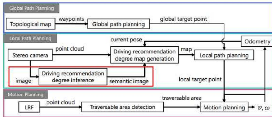
Fig. 5. Onozuka et al. Framework on Weakly Supervised Learning Traversability [101].
