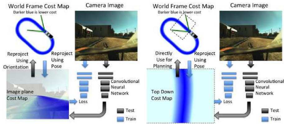
Fig. 6. The Framework of Automatic Labelling and Generating Cost Map [31].
