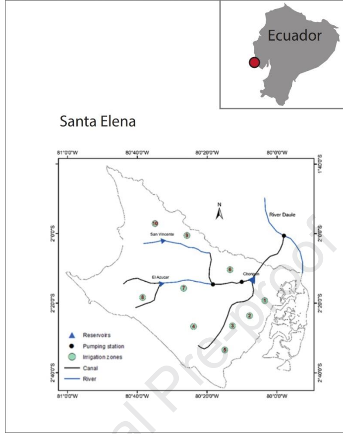
Figure 2 Schematic representation of the water infrastructure and irrigation zones in the SEP
