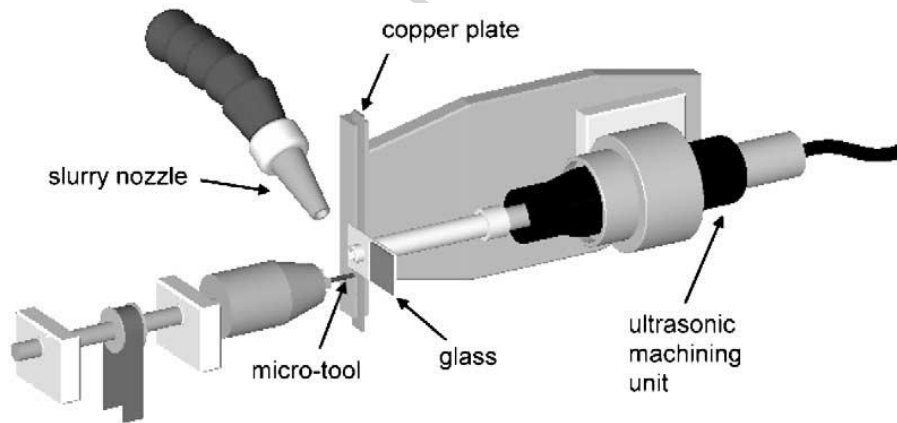
Fig. 11. A detailed diagram of experimental apparatus used in the MUSM process [12]
