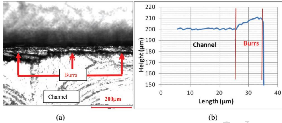
Fig. 25. Burrs left on the edge of the NAK80 microfluidic channels (a) SEM image of the burrs observed on the edge of the channel and (b) the profile of the channel [21]
