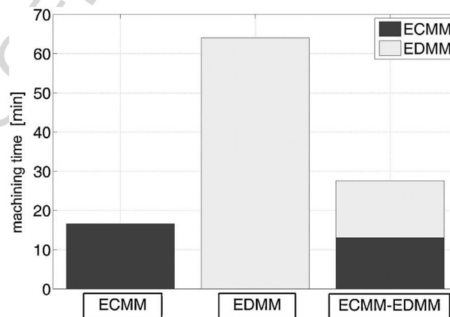
Fig. 14. Comparison of machining time [13]
