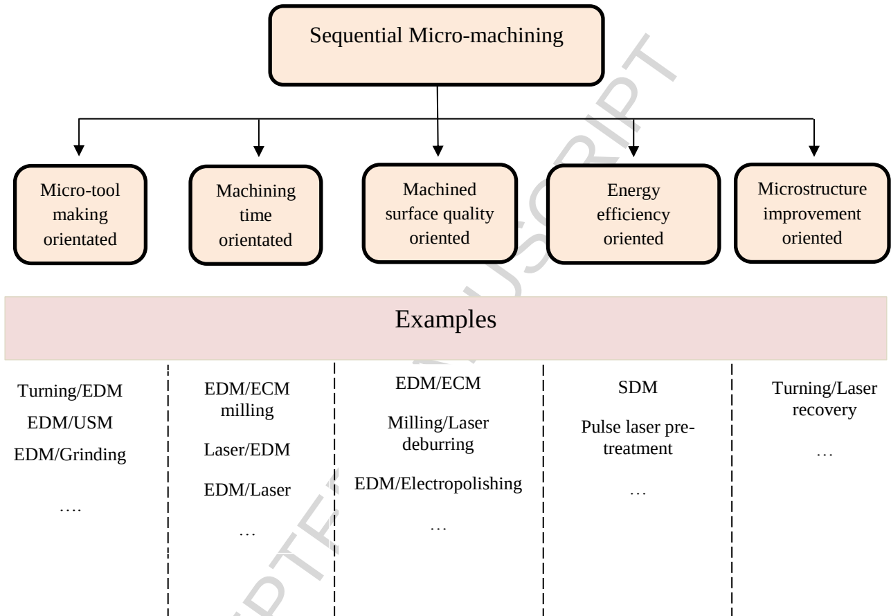
Fig 1. Classification of sequential micro-machining
