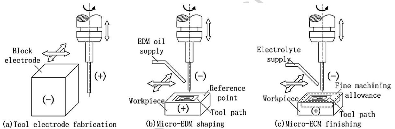
Fig. 22. Concept of block-EDM/ EDM/ ECM sequential machining process [20]
