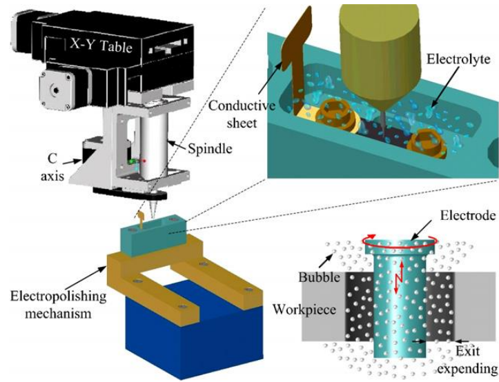
Fig. 28. Schematic diagram of electropolishing after micro-EDM [22]
