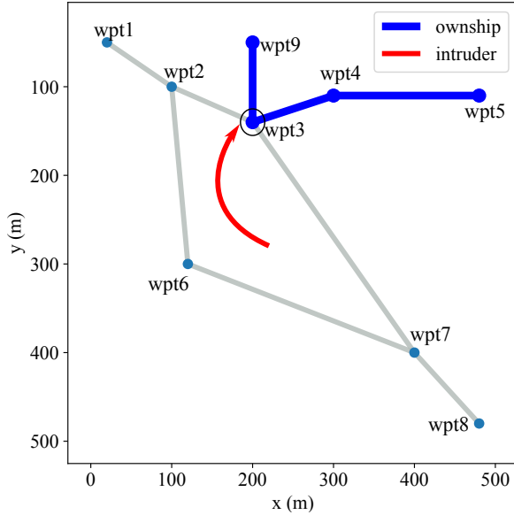
Fig. 4: Non-cooperative intruder.
