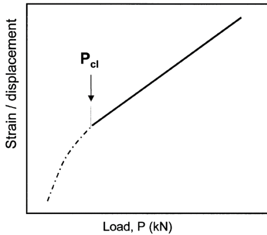
Fig.1 Schematic illustration of compliance curve based crack closure measurement.
