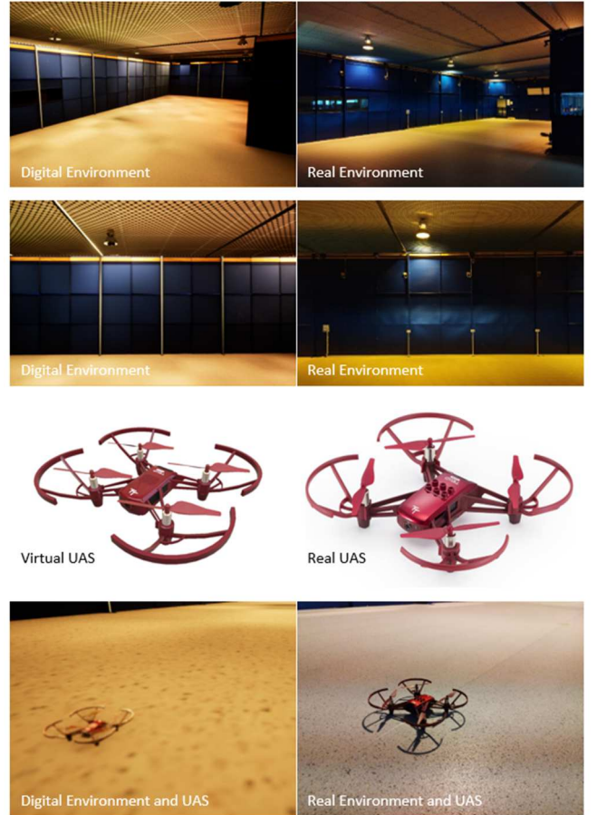
Fig. 9. Comparison of the digital environment and virtual UAS with their physical counterparts.
