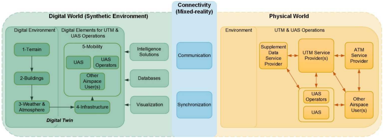
Fig. 3. Generic DT architecture, consisting of the digital world, the virtual world, and the connectivity between the two.
