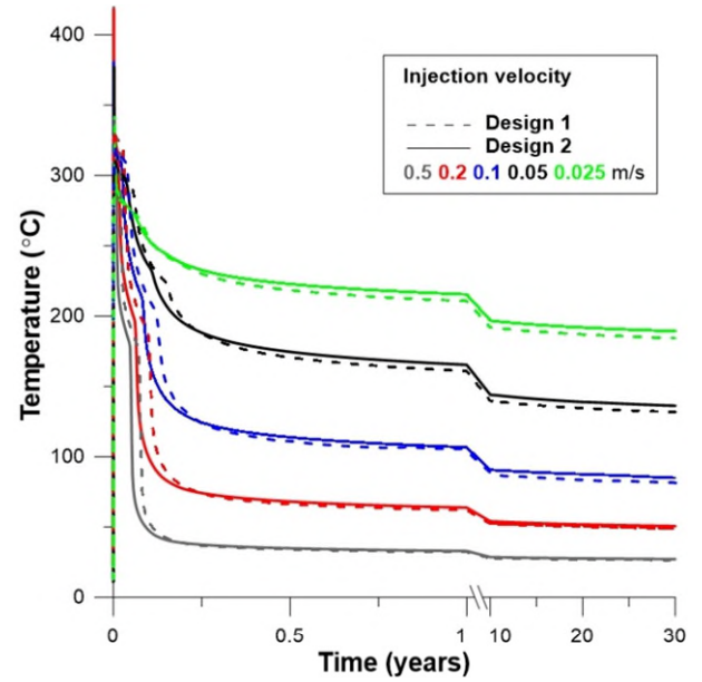
Figure 6: Production temperature over time, based on the injection velocity, until 30 years of simulation.
