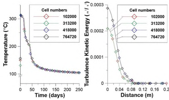
Figure 4: Transient outlet temperature (left) and radial turbulence kinetic energy (right) at 2008.1 m, with different meshes - Design 1.
