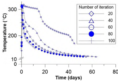
Figure 5: Outlet temperature over time based on the iterations per time step - Design 1.
