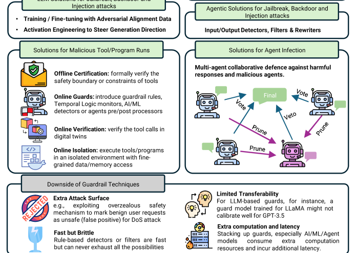
Fig. 3. High-level guardrail techniques for LLMs and agentic systems.
