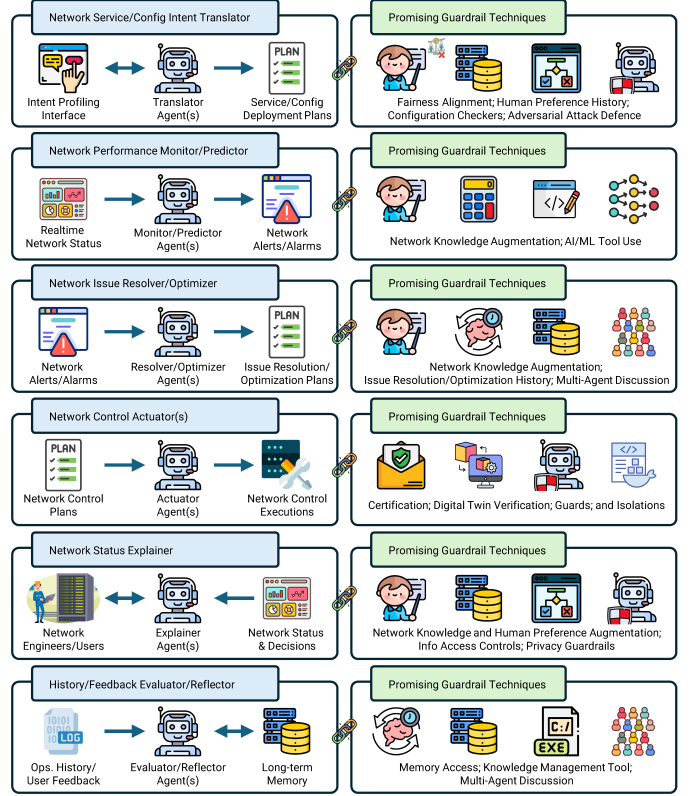
Fig. 4. LLM/Agent application patterns in 6G and promising guardrail techniques.
