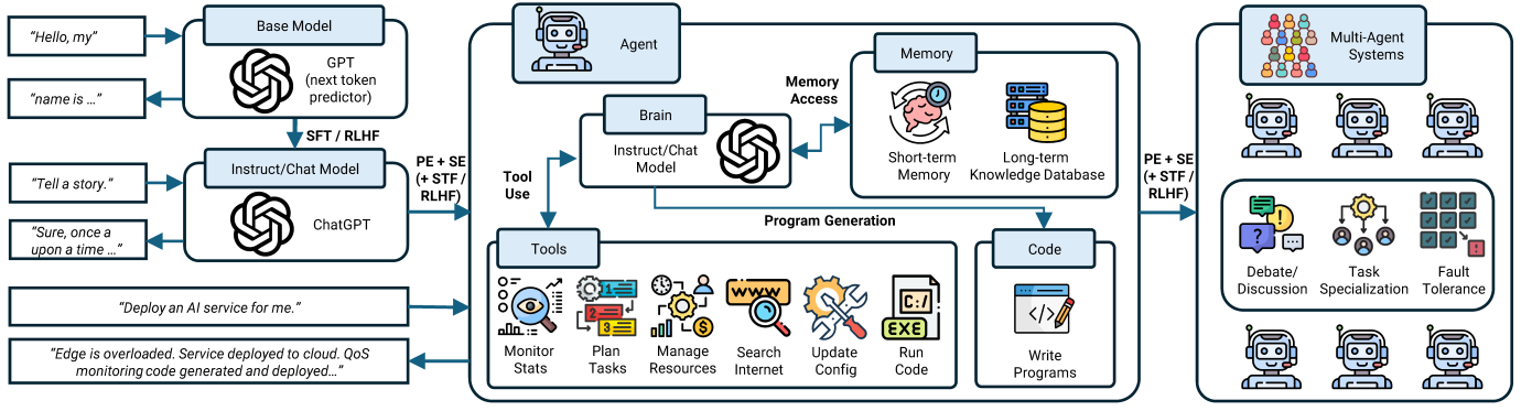
Fig. 1. From base models to multi-agent systems. SFT: Supervised Fine-tuning; RLHF: Reinforcement Learning with Human Feedback; PE: Prompt Engineering; SE: Software Engineering.
