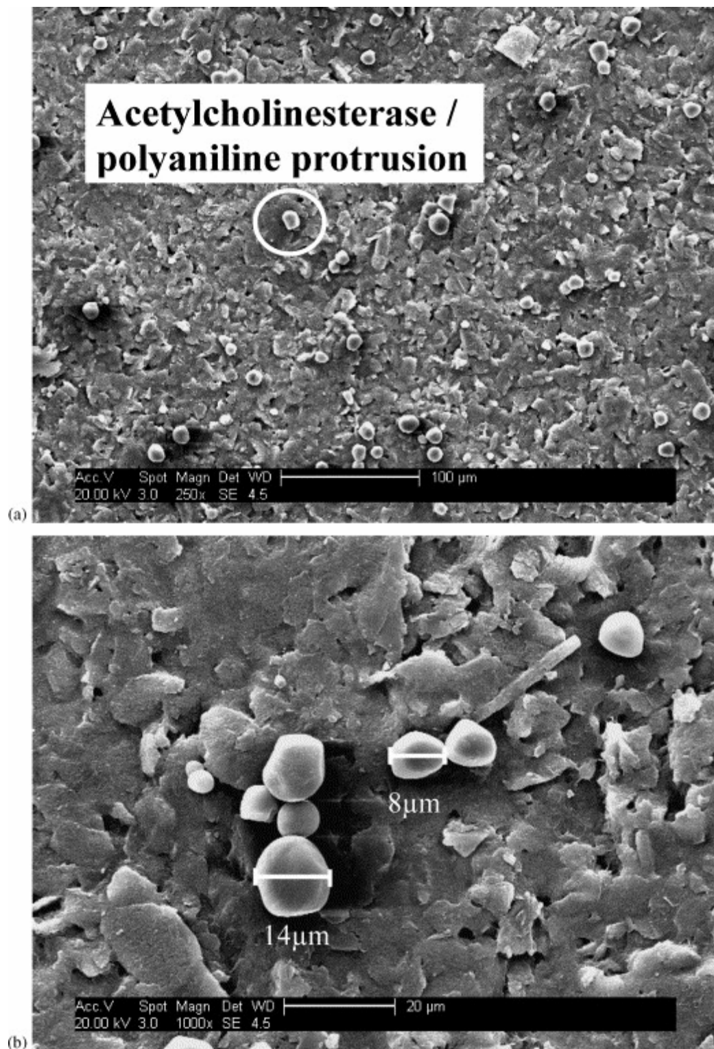
Fig. 2. Scanning electron micrographs of enzyme containing polyaniline protrusions at (a) 250 \times , (b) 1000 \times , (c) side view at an angle of 50 ^{\circ} 1000 \times , (d) side view 5000 \times .
