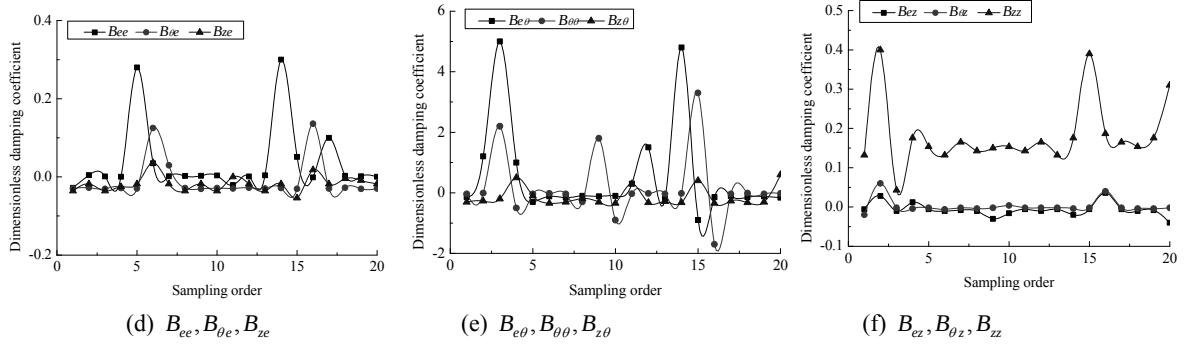
Figure 13. The gas film rotor instability of real time stiffness and damping coefficient of variation
