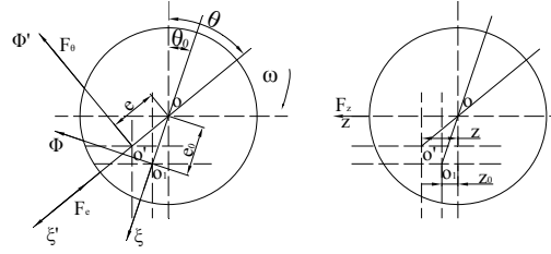
Figure 2. Rotor dynamic force diagram
