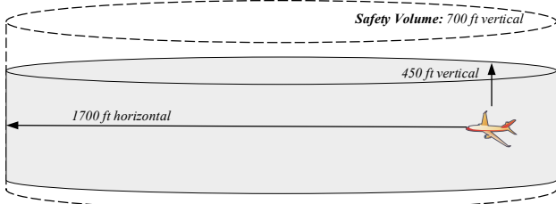
Fig. 8. CAA / FAR Safety Volume Definition
