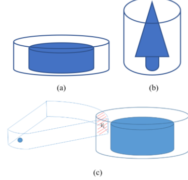
Fig. 5. Hazard assessment volumes representation: safety volume for static objects (a), safety volume for complex shapes (b), and intersection volume between sUAS safety volume (left) and static (c) object safety volume (right)
