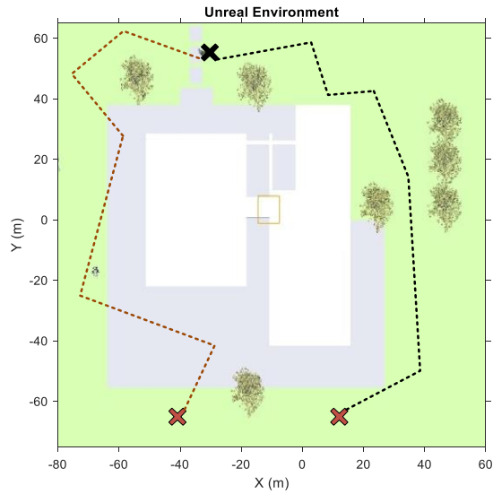
(a) Top View of Static Mesh Environment representing birds eye view of Fig.11 (a)
