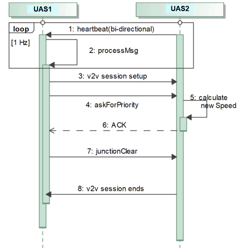
Fig. 1. Message exchange between UASs for collision avoidance.
