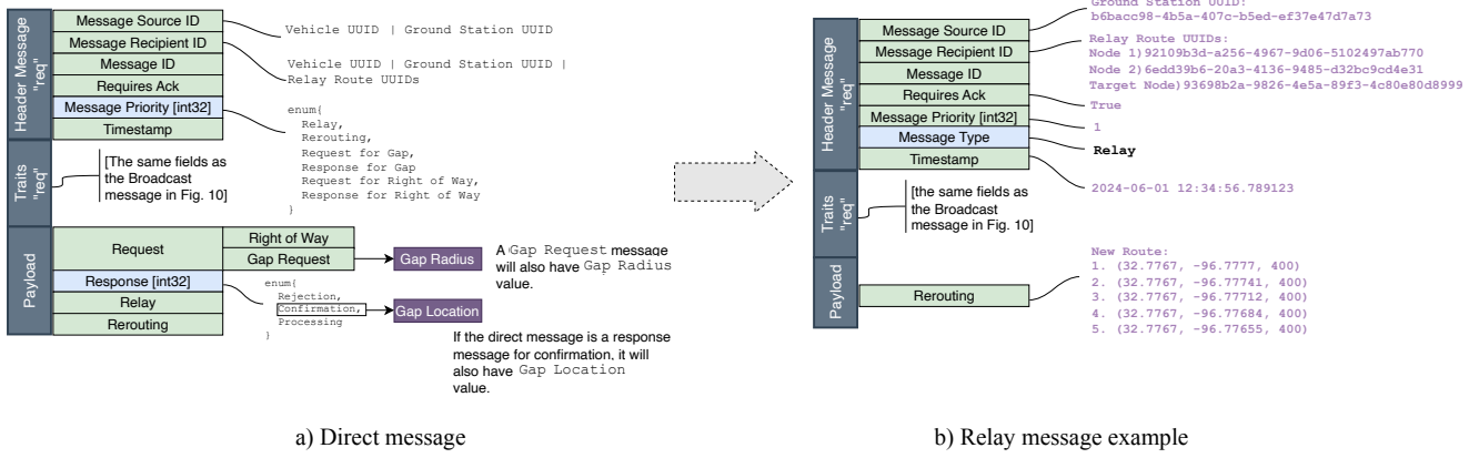
Fig. 4. Direct Message and a Relay message example showing how it is derived from a Direct Message.
