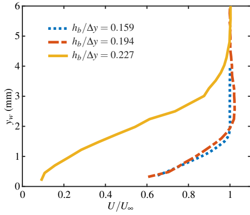
Figure 10: Boundary-layer profile at s/s_{\text{nac}} = 0.145 for different bump heights corresponding to variations in equivalent engine mass-flow rate: a) raw velocity profile; b) velocity values scaled by freestream velocity, U_\infty .
