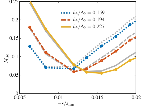
Figure 11: Pressure distribution on the internal nacelle surface around the stagnation point for different bump heights at a reduced entry Mach number, M_\infty = 0.60 . The gray lines correspond to the equivalent profiles at M_\infty = 0.65 .
