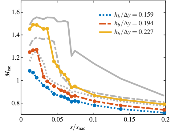
Figure 12: Pressure distribution on the external nacelle surface for different bump heights at a reduced entry Mach number, M_\infty = 0.60 . The gray lines correspond to the equivalent profiles at M_\infty = 0.65 .
