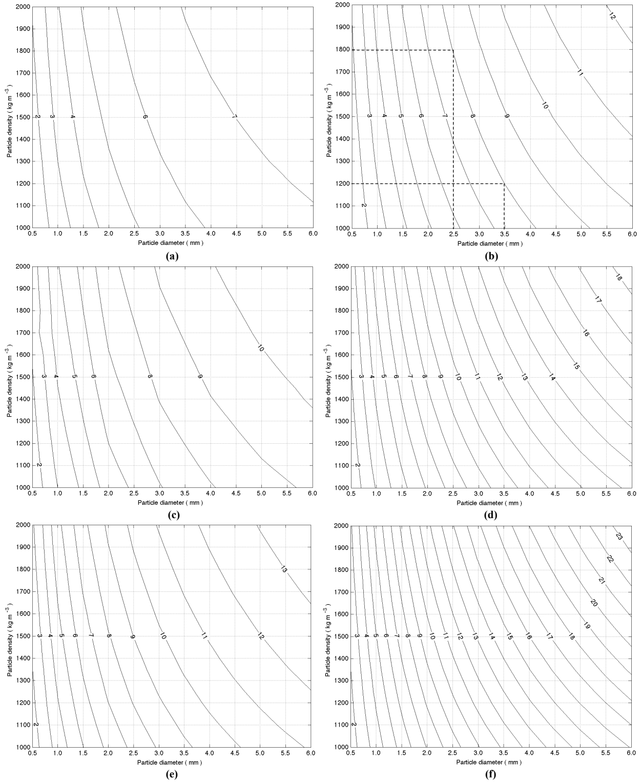
Figure 5. Contour plots used to determine landing distance of individual fertilizer particles based on particle diameter and particle density. Launch conditions are: h_0 = 1 \text{ m} , and (a): \alpha_0 = 0^\circ , v_0 = 20 \text{ m s}^{-1} , (b): \alpha_0 = 10^\circ , v_0 = 20 \text{ m s}^{-1} , (c): \alpha_0 = 0^\circ , v_0 = 30 \text{ m s}^{-1} , (d): \alpha_0 = 10^\circ , v_0 = 30 \text{ m s}^{-1} , (e): \alpha_0 = 0^\circ , v_0 = 40 \text{ m s}^{-1} , and (f): \alpha_0 = 10^\circ , v_0 = 40 \text{ m s}^{-1} . In (b), dashed lines illustrate the example given in the text for two fertilizer materials with d = 2.5 \text{ mm} and \rho_p = 1800 \text{ kg m}^{-3} , and d = 3.5 \text{ mm} and \rho_p = 1200 \text{ kg m}^{-3} , respectively.
