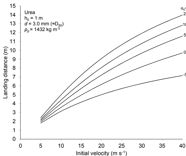
Figure 4. The effect of launch angle and initial velocity on landing distance of individual fertilizer particles. Particle density used in calculations is representative of urea with particle diameter equivalent to D_{50} .
