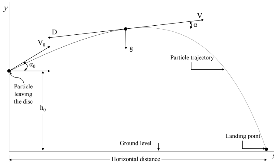
Figure 1. Trajectory and forces acting on a fertilizer particle after leaving a spinner disc.
