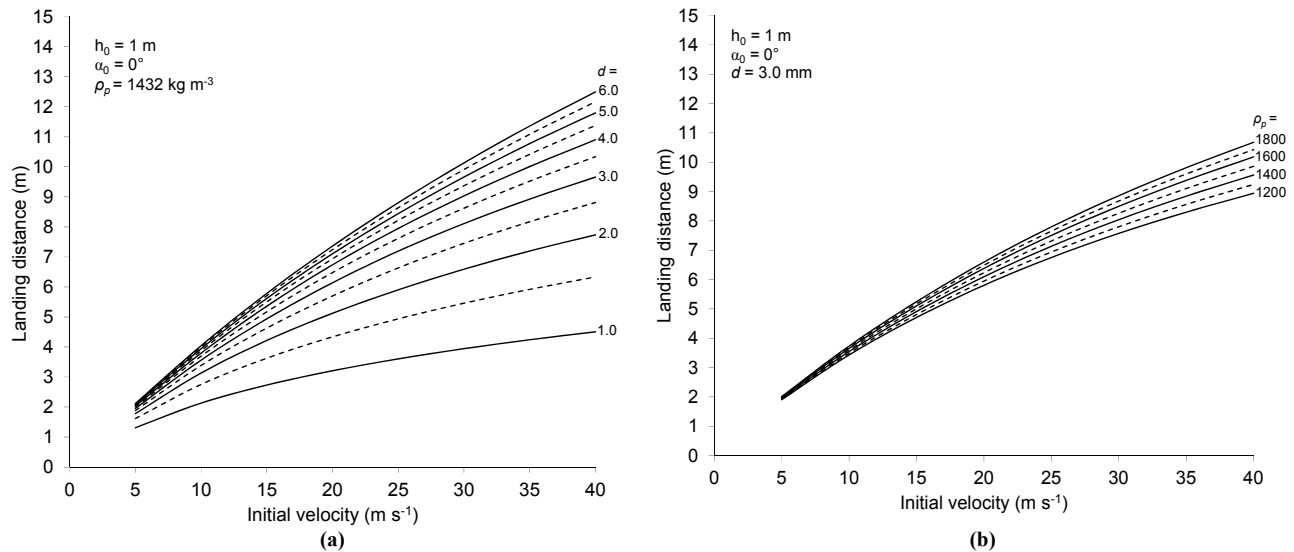
Figure 3. The effects of (a) particle diameter and initial velocity, and (b) particle density and initial velocity on landing distance of individual fertilizer particles. Dashed lines represent responses for intermediate values of particle diameters or particle densities, respectively.
