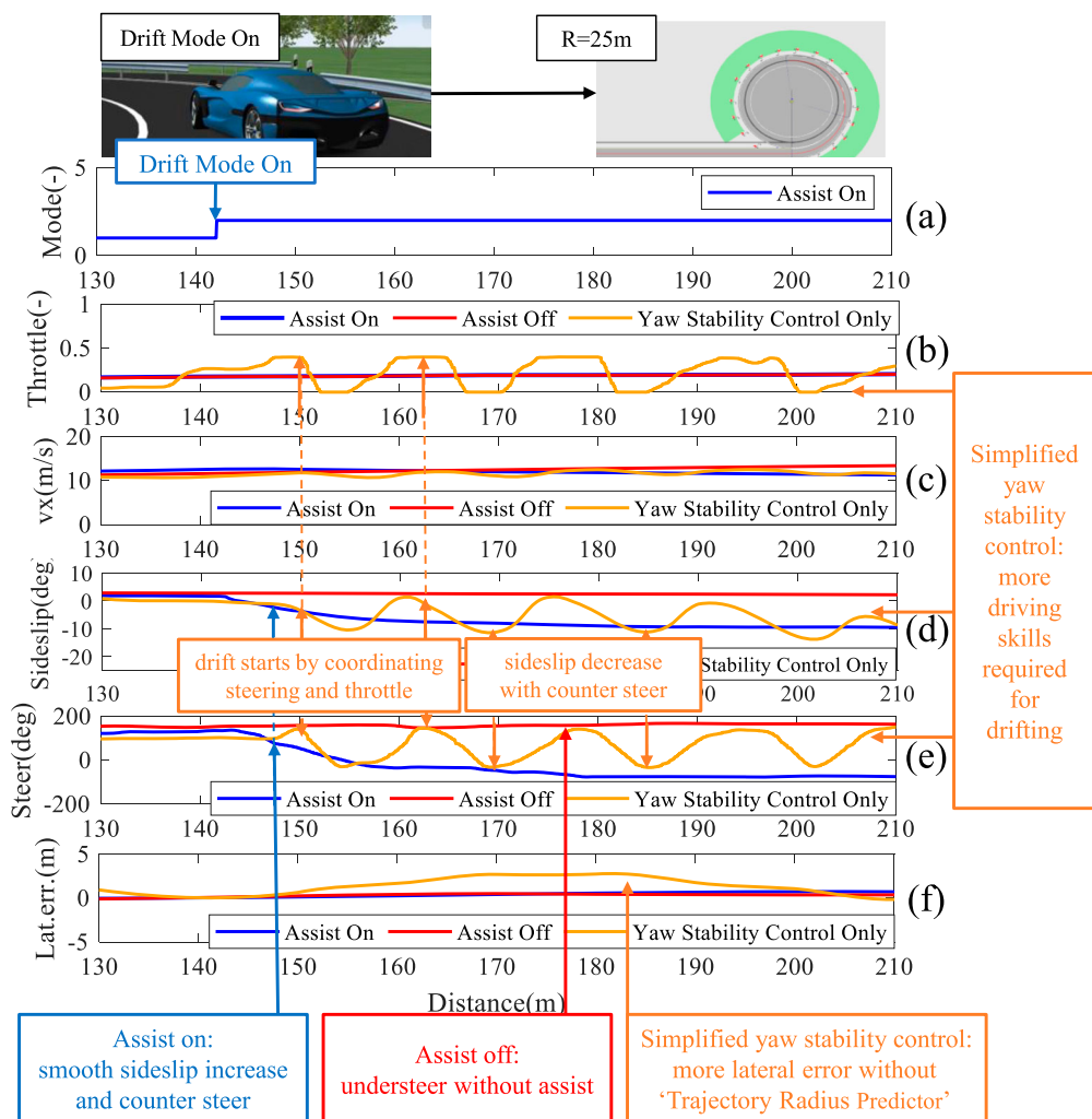
Figure 6. Simulation results of drift assist control on/off, and additional comparison with a simplified yaw stability controller on a fixed radius track.
