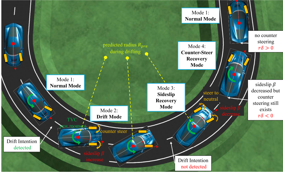
Figure 2. The transition between four drive modes in a corner.
