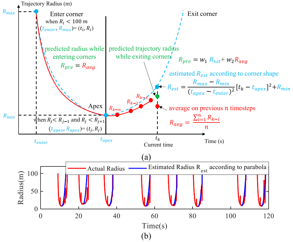
Figure 3. The trajectory radius predictor (a) and the estimated radius R_{est} in the exit of corners on a rally track according to parabola (b).
