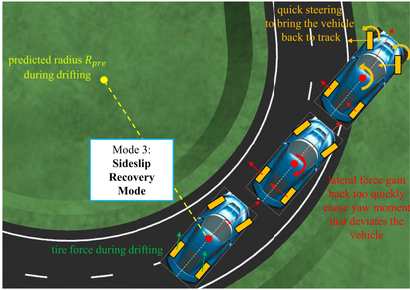
Figure 4. Why the rear axle should not gain back lateral force too quickly in Mode 3.
