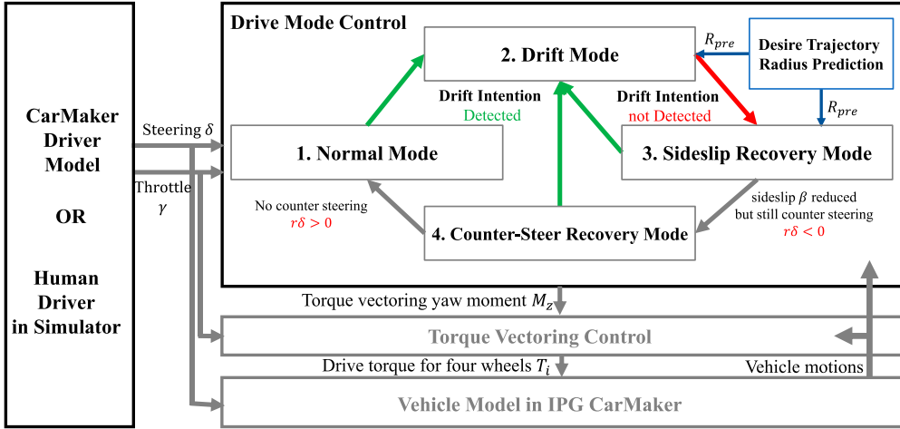
Figure 1. The proposed control framework.
