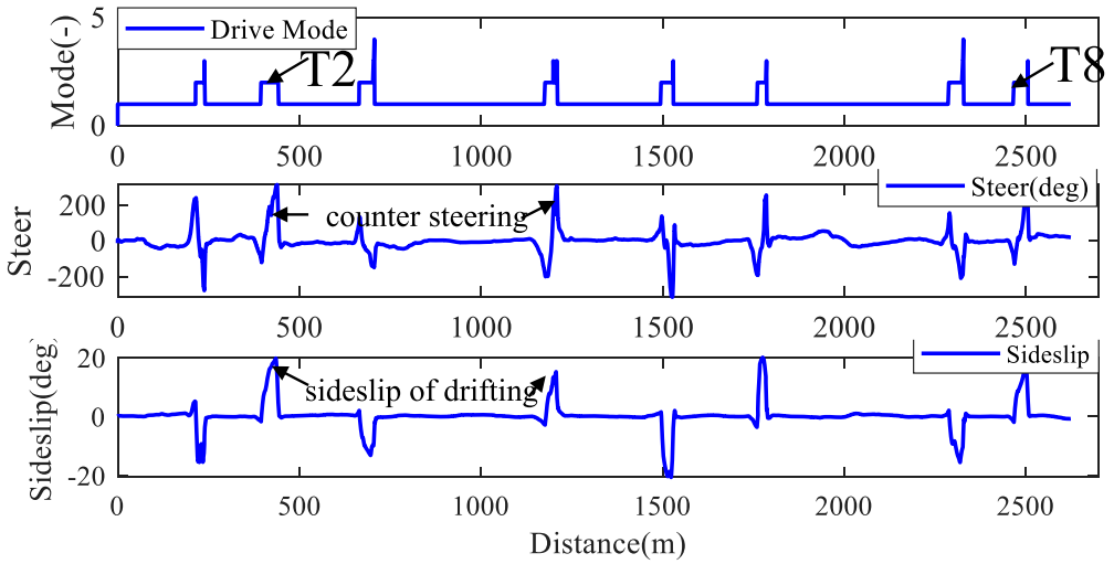
Figure 13. The drive mode transition and sideslip on Pikes Peak with a human driver (video at: https://www.youtube.com/watch?v=02aSdIMkZlg ).
