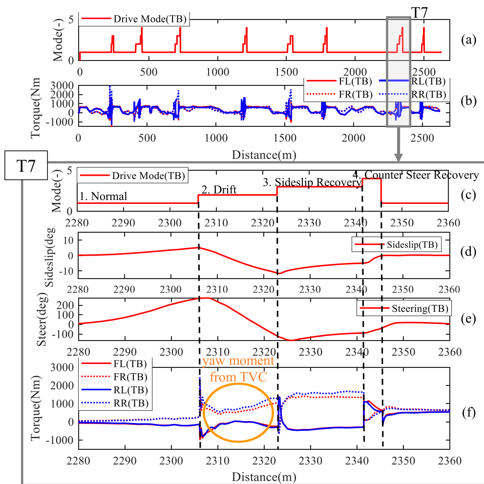
Figure 11. The wheel torque during the seventh corner (T7) on Pikes Peak with TB cornering (video at: https://www.youtube.com/watch?v=oW0LCQXVhJQ ).
