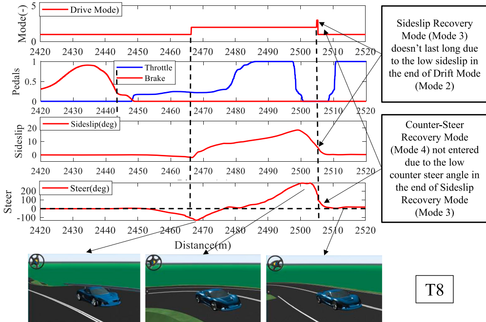
Figure 14. The vehicle behaviour at T8 of Pikes Peak with human driver.
