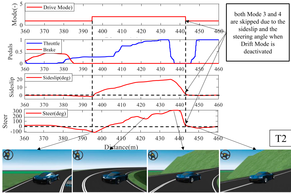
Figure 15. The vehicle behaviour at T2 of Pikes Peak with human driver.
