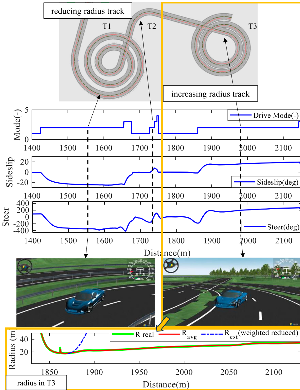
Figure 8. Simulation results with drift assist control on varying radius track (video at: https://www.youtube.com/watch?v=7preJkxoRe8 ).
