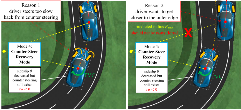
Figure 5. The reasons behind the abnormal counter steering after entering Mode 4.
