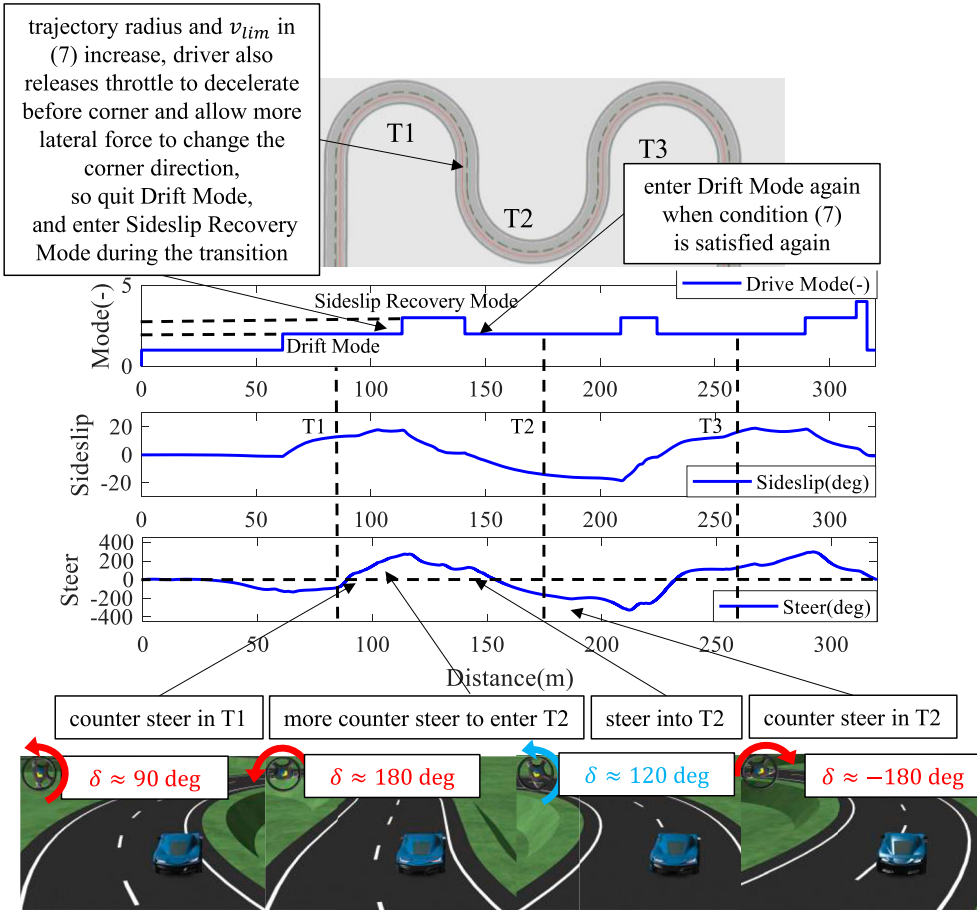
Figure 7. Simulation results with drift assist control on S-Turn track (video at: https://www.youtube.com/watch?v=1p8AyHKGk8 ).
