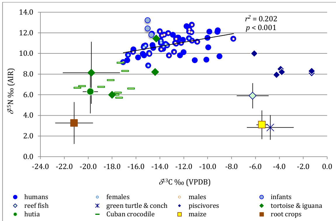
Figure 4. Relationship between \delta^{13}\text{C} and \delta^{15}\text{N} values for Bahamian humans and comparative fauna and adjusted flora (for details see S1.4; error bars are \pm 1\text{SD} ). The regression line ( r^2 = 0.202 , p < 0.001 , n = 61 ) excludes the three infants, potentially subject to a nursing effect. The large blue circles represent all post-weaning humans, with the smaller inset symbols identifying sex where available. The Bahamian results stand out in a comparison with other Caribbean islands in their higher average \delta^{13}\text{C} values, interpreted as reflecting greater use of reef resources (Table S6, Figure S3).
