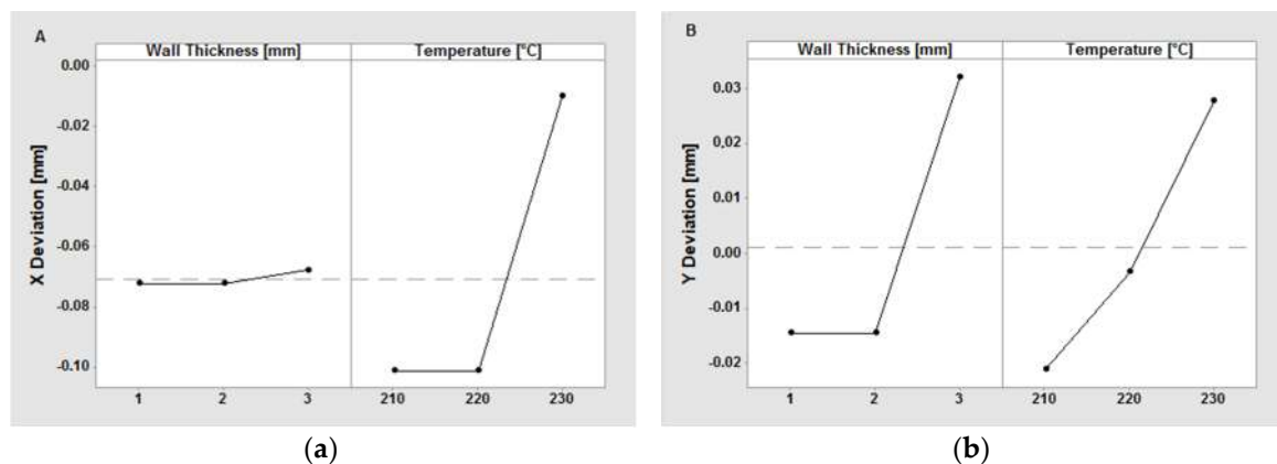
Figure 4. Plot of means for dimensional deviation for (a) the X dimension and (b) the Y dimension.
