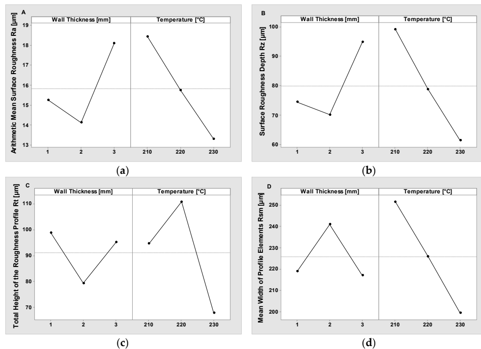
Figure 5. Plot of means for surface roughness parameters: (a) arithmetic mean surface roughness Ra, (b) surface roughness depth Rz, (c) total height of the surface roughness profile Rt, and (d) mean width of profile elements Rsm.
