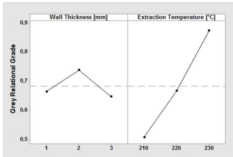
Figure 6. Plot of means for grey relational grade.
