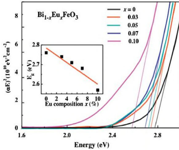
Fig. 10. (\alpha E)^2 plotted as function of photon energy for \text{Bi}_{1-x}\text{Eu}_x\text{FeO}_3 ( x = 0, 0.03, 0.05, 0.07, 0.10 ) films. The inset shows the variation of the optical band gap of \text{Bi}_{1-x}\text{Eu}_x\text{FeO}_3 films [78]. Copyright 2014 Elsevier Ltd.
