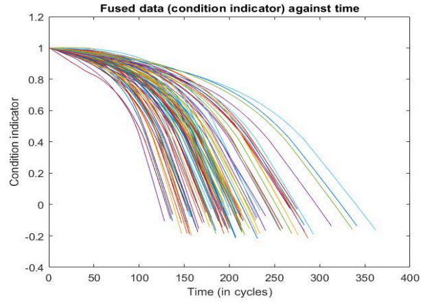
Fig. 9. Constructed HIs using trained data for all 100 units within the fleet.
