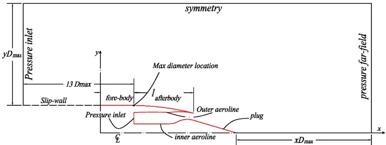
Figure 2 Boundary domain and boundary conditions of the nozzle CFD simulations.
