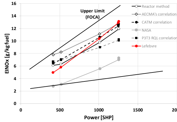
Figure 12: EI \text{NO}_x prediction for different power settings of the T700-GE-700 model
