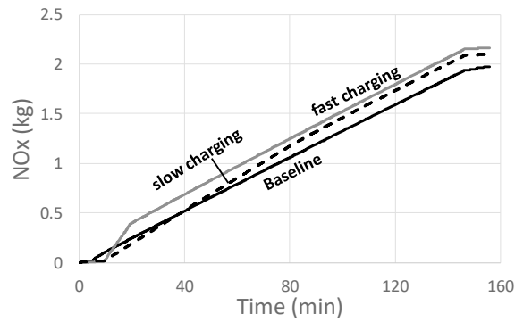
Figure 19: \text{NO}_x pollutant emissions for fast and slow recharging for Case C; PMS1
