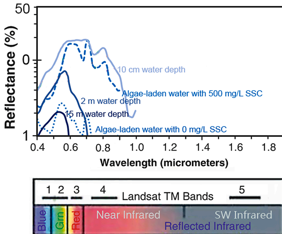
Fig. 2. Spectral bands and reflectance of various substance including water modified after Schowengerdt (2007) considering work of Han (1997), Lafon et al (2002). This is showing various influence of reflectance of water. Note that Y axis is in logarithmic scale.
