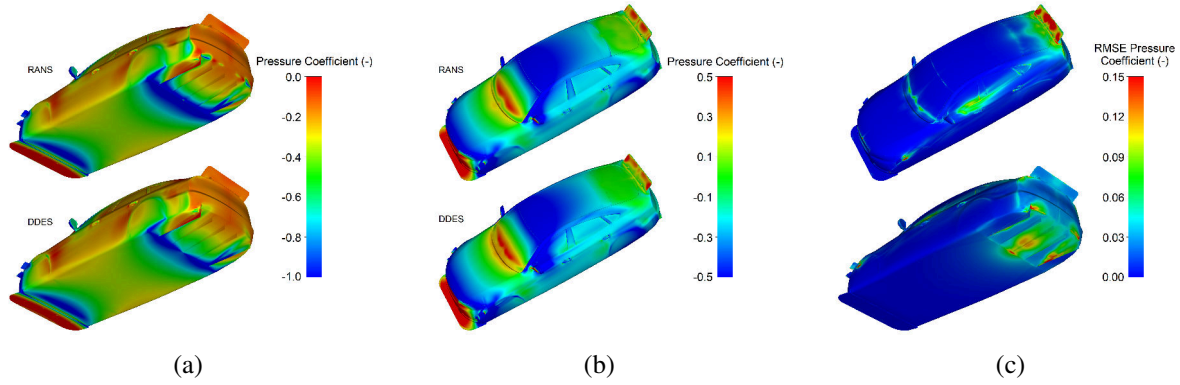
Figure 2: Mean pressure coefficient at the (a) underbody and (b) upper surface, and (c) Root Mean Square Error (RMSE) for the mean pressure coefficient of the DDES simulation
