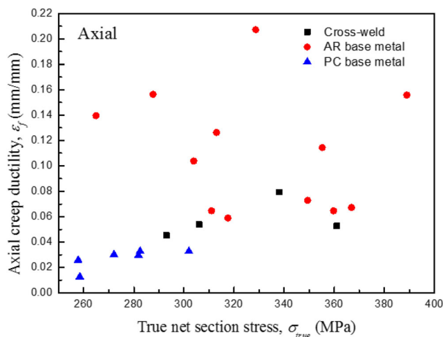
Fig. 12 Axial creep ductility vs. true stress for the XW, AR and PC materials
