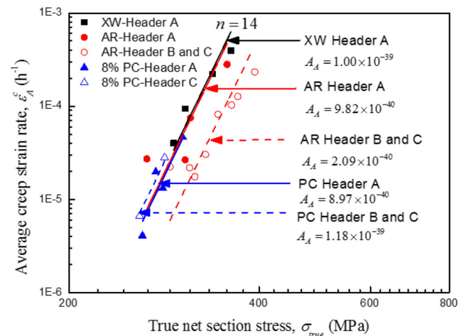
Fig. 16 Comparison of the average creep strain rate trends for the XW, PC and AR specimens
