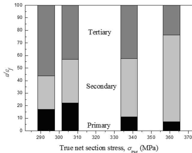
Fig. 8 Relative percentage of strain accumulated in each creep region for cross-weld specimens
