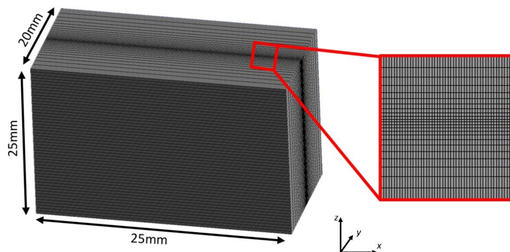
Figure 7. Model dimensions setup and mesh design.
