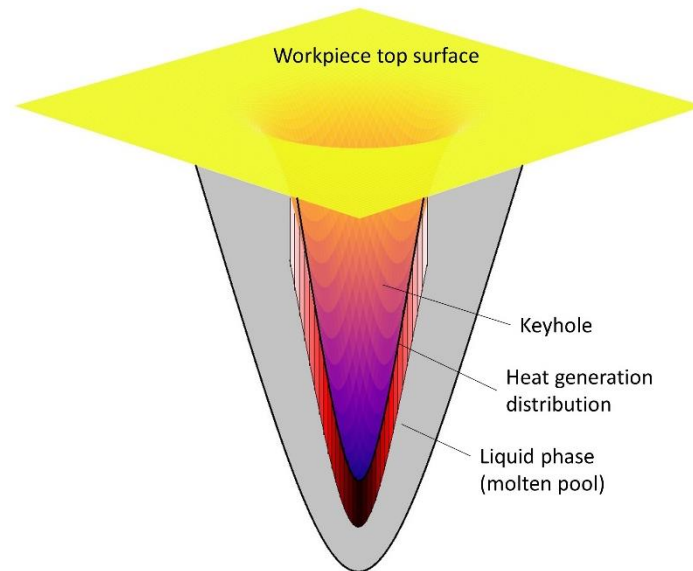
Figure 8. Sketch of heat source generation, with darker red representing higher energy density and vice versa.
