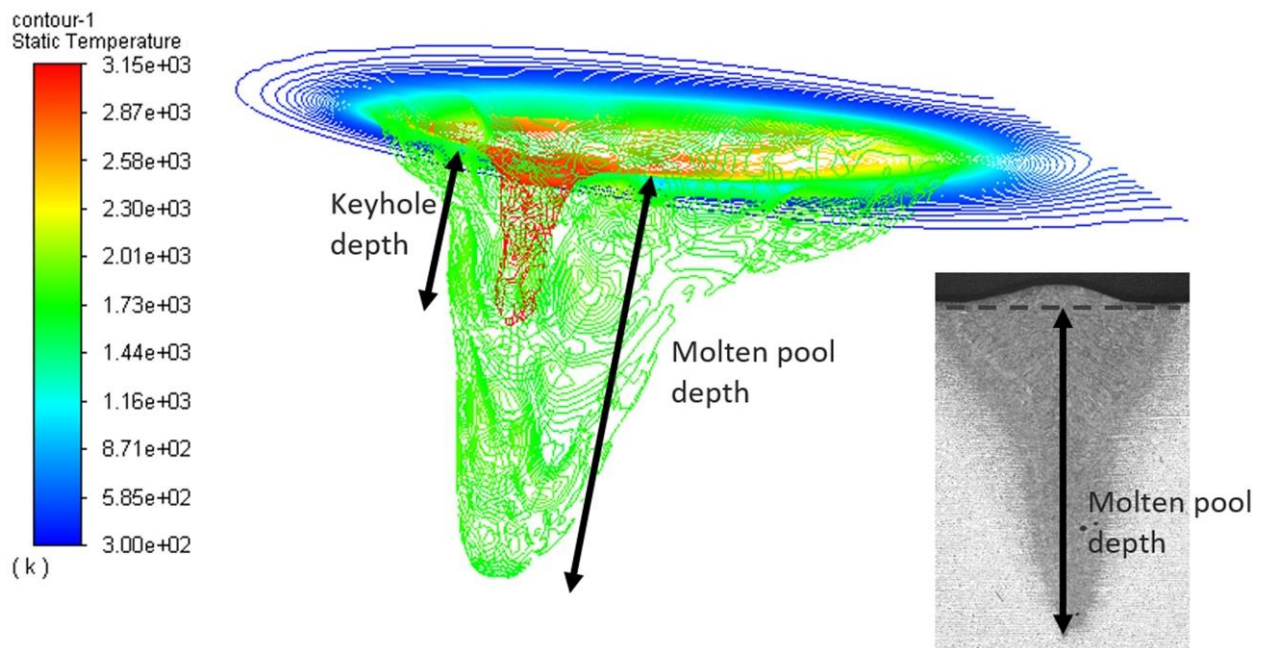
Figure 9. An example of molten pool penetration depth prediction using the CFD method.
