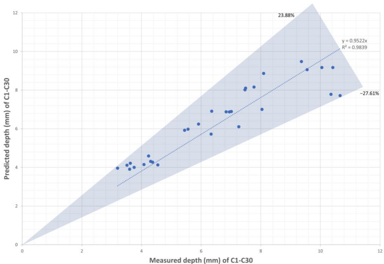
Figure 13. Predicted depths by CFD-based BPNN compared with measured depths of C1–C30.
