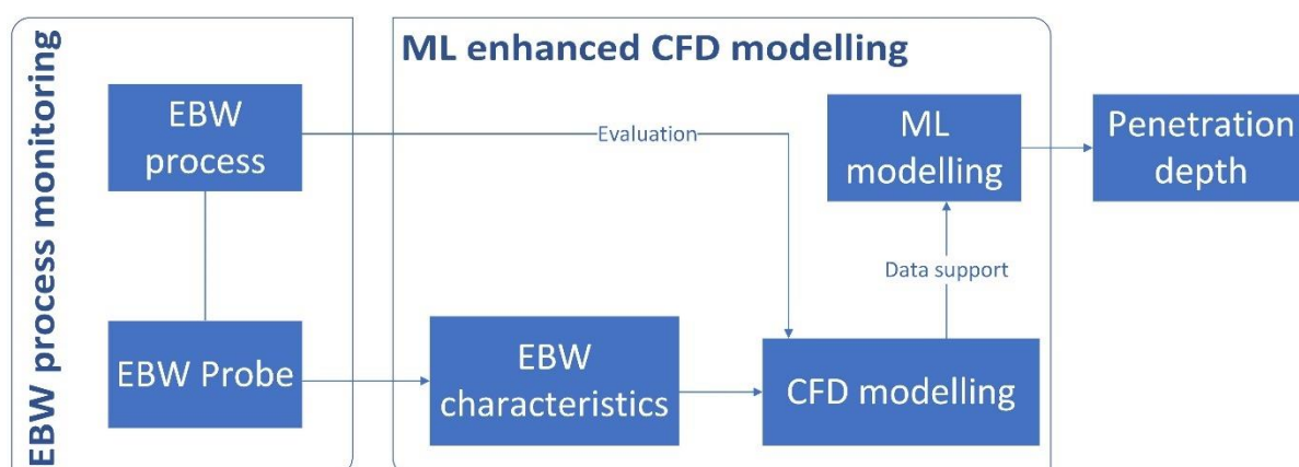
Figure 1. Schematic diagram of ML enhanced CFD modelling for EBW penetration depth prediction.
