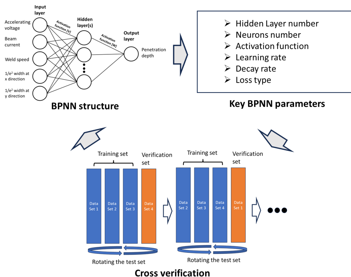
Figure 10. Procedure to determine BPNN structure and parameters.
