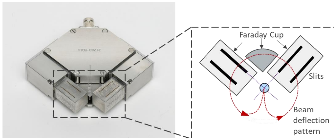
Figure 4. Modified 4-slit probe developed by TWI Ltd., Cambridge, UK.
