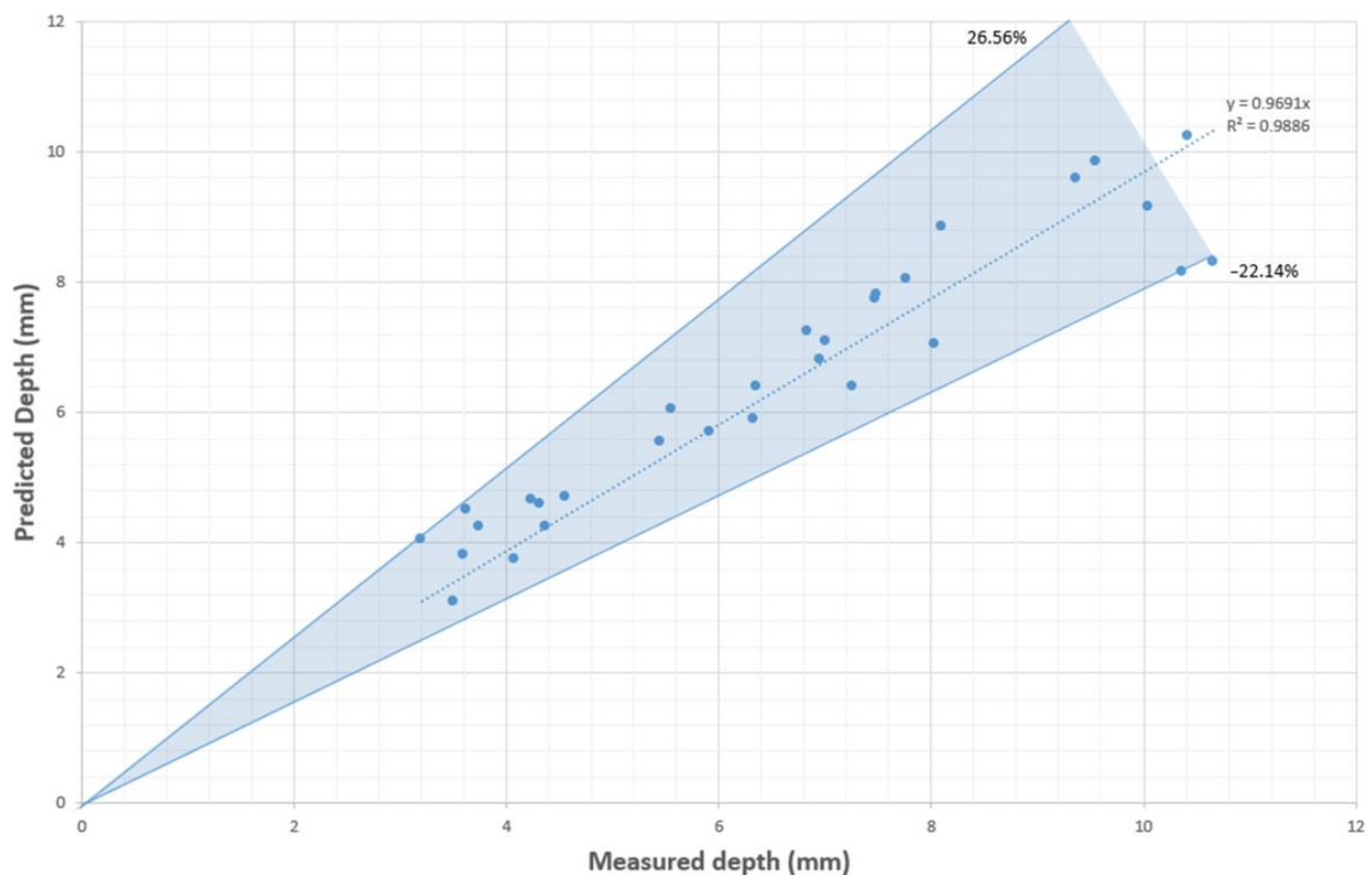
Figure 11. Simulated depths via CFD modelling compared with measured depths of C1–C30.
