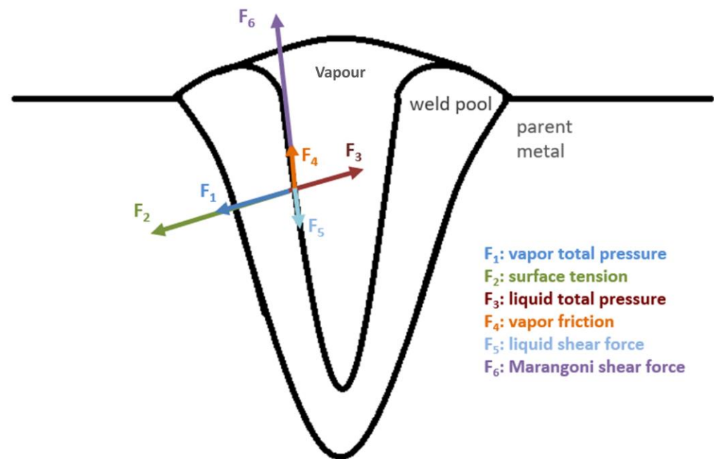
Figure 6. Primary forces operating at the molten pool interface during EBW.
