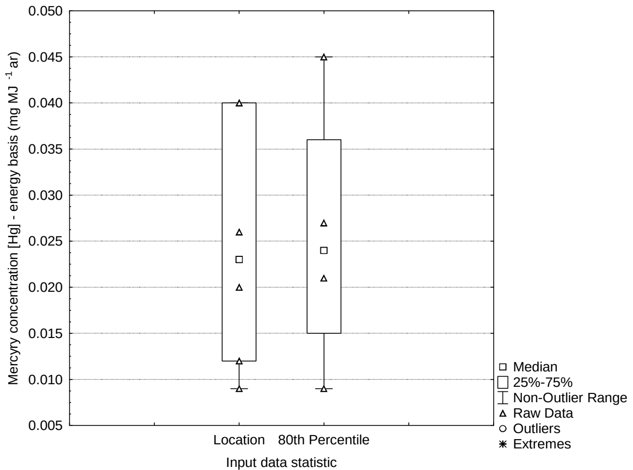
FIGURE 26 Results of descriptive statistical analysis on MBT-derived SRF data:
