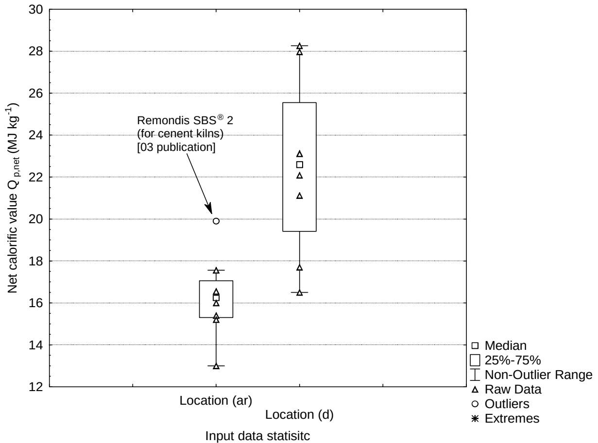
FIGURE 20 Results of descriptive statistical analysis on MBT-derived SRF data:
