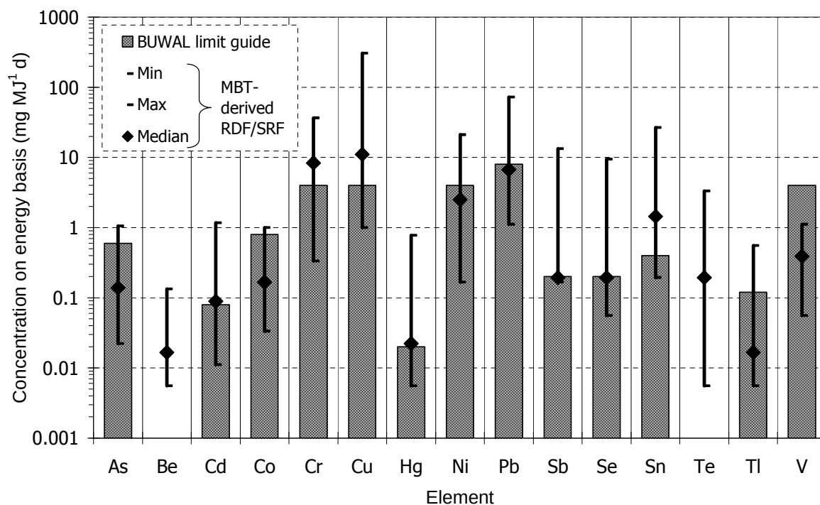
FIGURE 19 Energy-based concentrations of trace elements in RDF produced in early MBT plants, presented on logarithmic scale. Comparison with the 1998 limit guidance concentrations of the Swiss Agency for the Environment, Forrester and Landscape (BUWAL). A Q_{p,net} of 18 MJ kg -1 has been assumed to convert values from mass basis to energy basis. Redrawn from Rotter et al. 49
