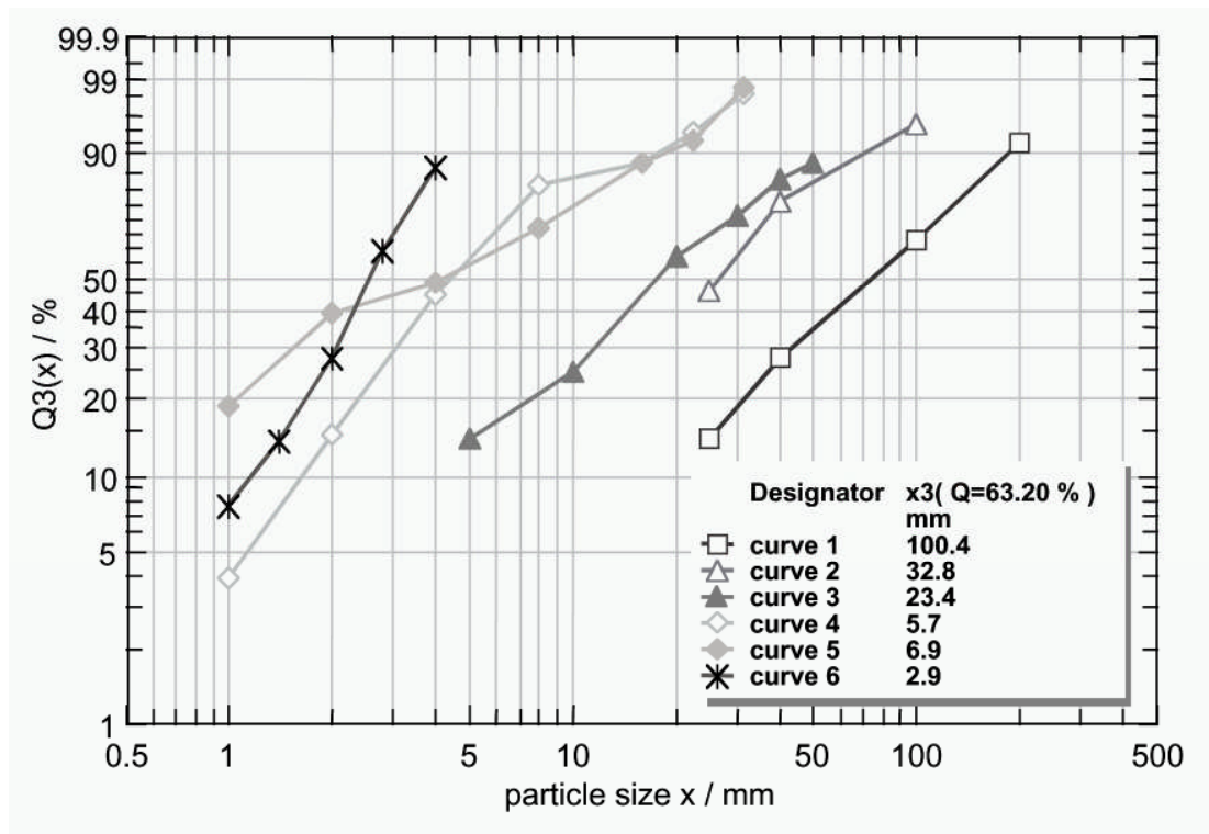
FIGURE 10 Cumulative mass fractions reporting at the screen undersize for various types of pre-treated domestic waste. Curves: (1) feed material; (2) comminution and drum screen at 100 mm; (4) and (5): ball-mill and 40 mm trommel underscreen; (6) ball mill-trommel and separation <5 mm organic-rich fraction. Characteristic particle size d_{63.2} values are provided (63.2% w/w total mass smaller in size). From Koch et al. 145 , with permission
