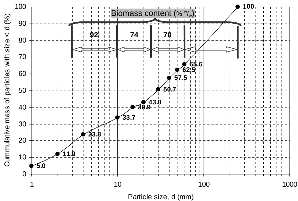
FIGURE 17 Particle-size distribution by sieve analysis of Herhof SRF (Stabilat®). Fractions with particle size lower than 60 mm exhibit high biomass content. Redrawn from Wengenroth 168
