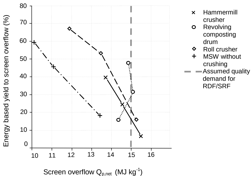
3647 FIGURE 9 Effect of comminution and screening on the relationship of net calorific value
