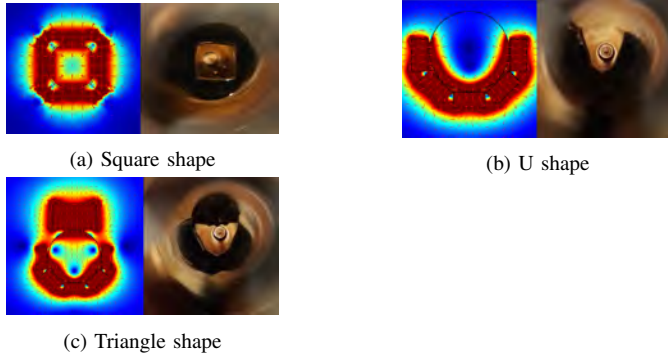
Fig. 9: Valve shape design
