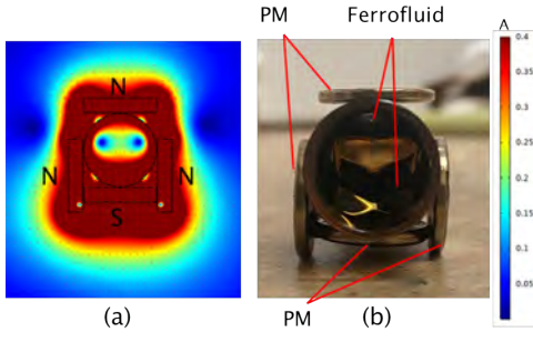
Fig. 8: Fig. 8: Shape prediction of ferrofluid (a) FEM model (b) Experimental
