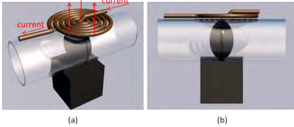
Fig. 2: (a):Schematic model of ferrofluid valve (valve off, excitation on), (b): Side elevation.
