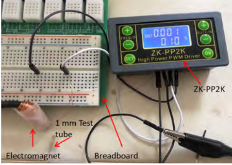
Fig. 3: Experiment set-up.
