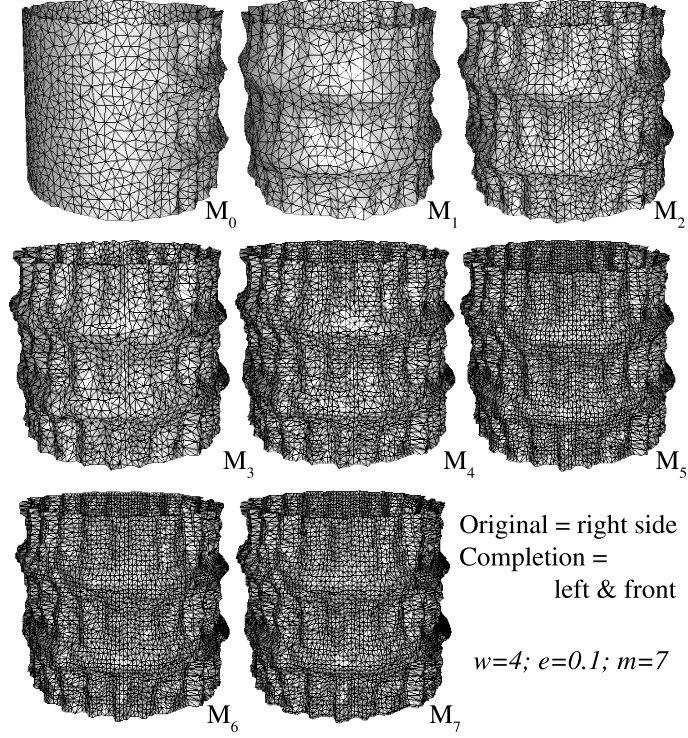
Figure 11. Stages of hierarchical completion for Figure 10
