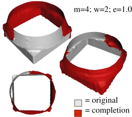
Figure 15. Hierarchical completion of non-conforming plinth
