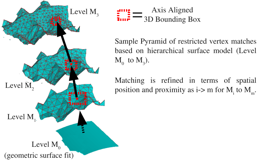
Figure 5. Sample pyramids for restricted matching
