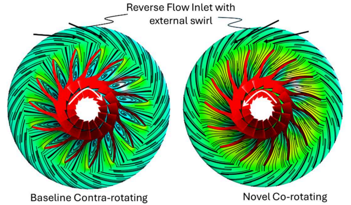
Fig.18 Notional maximum potential power production case in the contra-rotating and co-rotating mode with externally induced swirl
