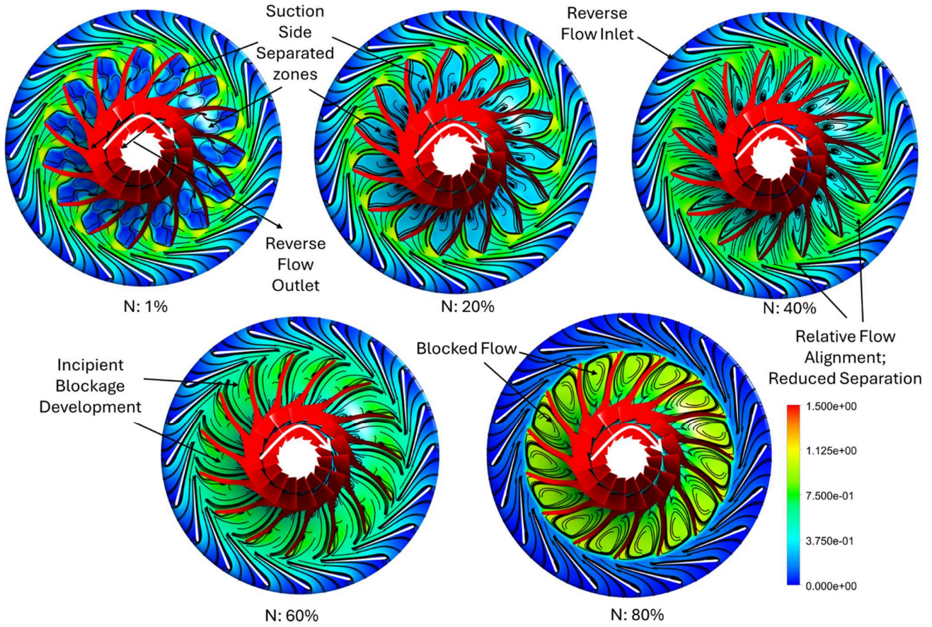
Fig.10 Streamlines on the 50% blade-to-blade section colored with a Mach number color palette for different rotational speeds in the baseline contra-rotating turbine mode – rotation direction marked in white arrows. Note on color bar – Red does not occur in contours. Impeller is colored red for contrast.
