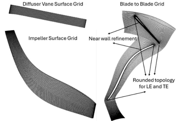
Fig. 5 Representative grids used in the analysis with key features highlighted.
