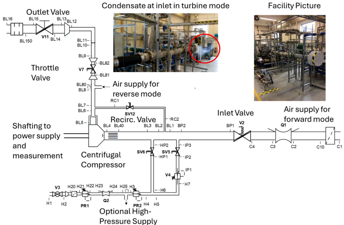
Fig.19 Experimental facility layout for reverse flow contra-rotating mode investigations. Picture of the facility shown in insert.
