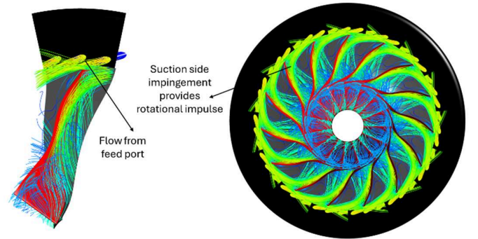
Fig.16 3D streamlines in the feed port architecture for N:1% in the novel co-rotating turbine mode.
