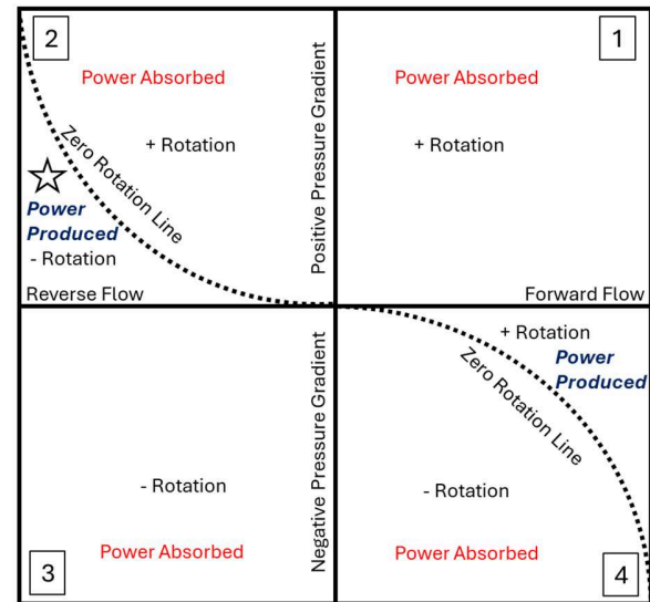
Fig. 2 Representative four-quadrant compressor operation map. Image reconstructed as adapted from [8].
