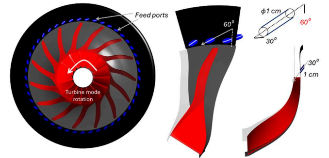
Fig.8 Feed port arrangement with directed holes to enable co-rotating turbine mode operation.
