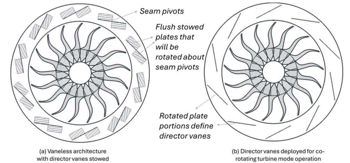
Fig.7 Exemplary mechanical arrangement for deploying director vanes in vaneless architectures.
