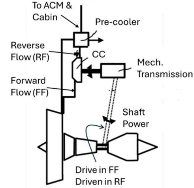
Fig. 1 Schematic of EMC 2 S Architecture showing ECS mode in Forward Flow (FF) and starting mode in Reverse Flow (RF)
