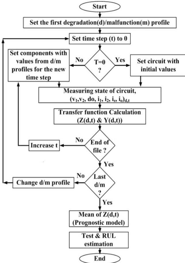
Fig. 5. Algorithm used to develop prognostic model. d/m : degradation/mulfunction number; t : time step or cycle.
