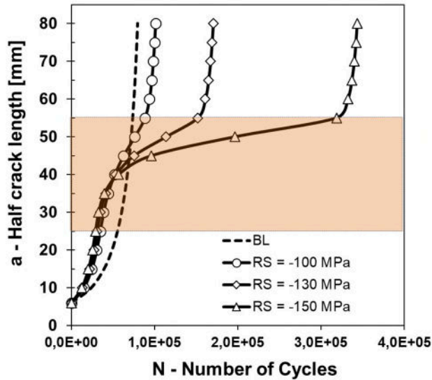
Figure 14 Crack length – cycles data for 3 different values of \sigma_{res} = -100, -130, \text{ and } -150 \text{ MPa} ; d_{lp} = 20 \text{ mm} , w_{lp} = 30 \text{ mm} .
