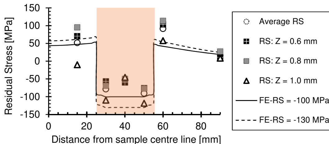
Figure 16 Comparison of measured and calculated residual stresses in peened sample of 1.6 mm 2524 aluminium; d_{lp} = 25 mm, w_{lp} = 30 mm.
