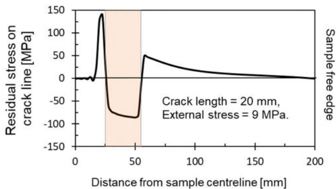
Figure 9(a) Uncracked residual stress field; external stress of zero.
