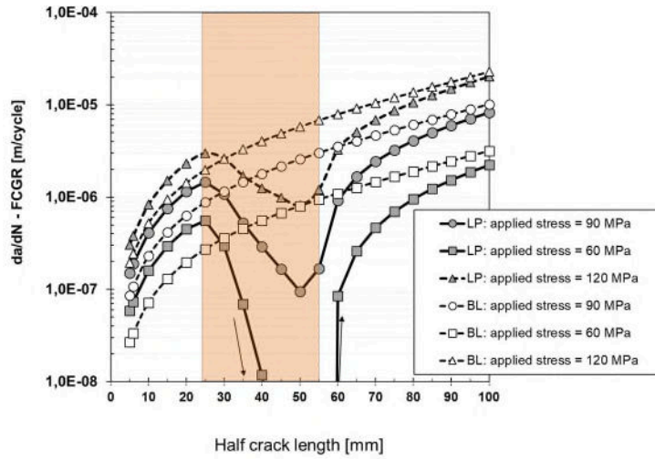
Figure 12 Effects of external cyclic stress on da/dN ; Comparison of da/dN changes for \sigma_{\max} = 60, 90 and 120 MPa; \sigma_{\text{res}} = -130 MPa, d_{\text{lp}} = 25 mm, w_{\text{lp}} = 30 mm.
