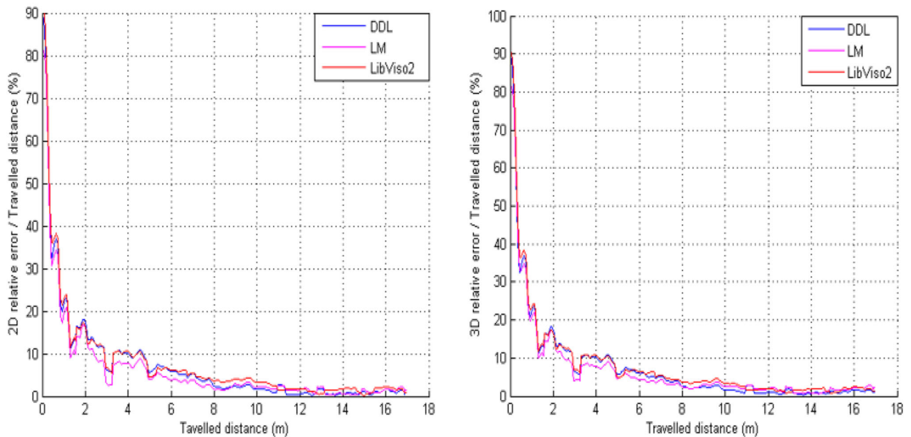
Fig. 12 Run A: relative RMSE 2D ( left ) and 3D ( right ) in per cent over the travelled distance regarding the Vicron reference trajectory
