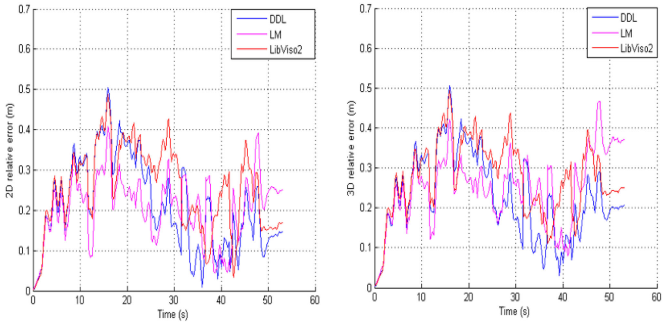
Fig. 11 Run A: relative RMSE 2D ( left ) and 3D ( right ) in metre over the time regarding the Vicron reference trajectory
