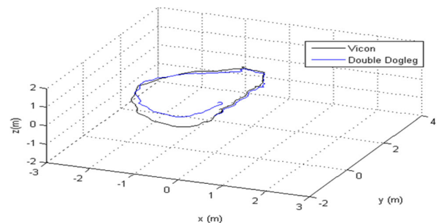
Fig. 14 Run B: 3D plot of the trajectory generated with the navigation sensor using the double-dogleg algorithm ( blue ) compared to the Vicon reference ( black )
