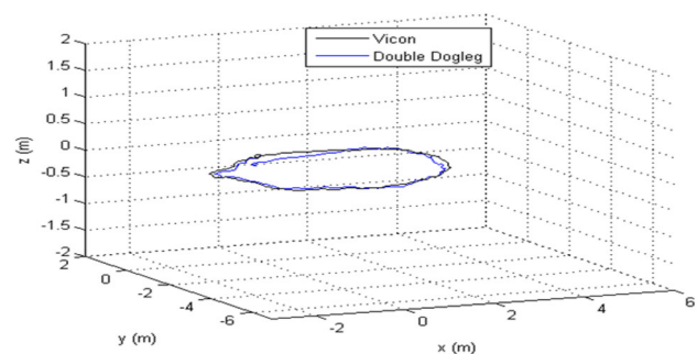
Fig. 10 Run A: 3D plot of the trajectory generated with the navigation sensor using the double-dogleg algorithm ( blue ) compared to the Vicon reference ( black )
