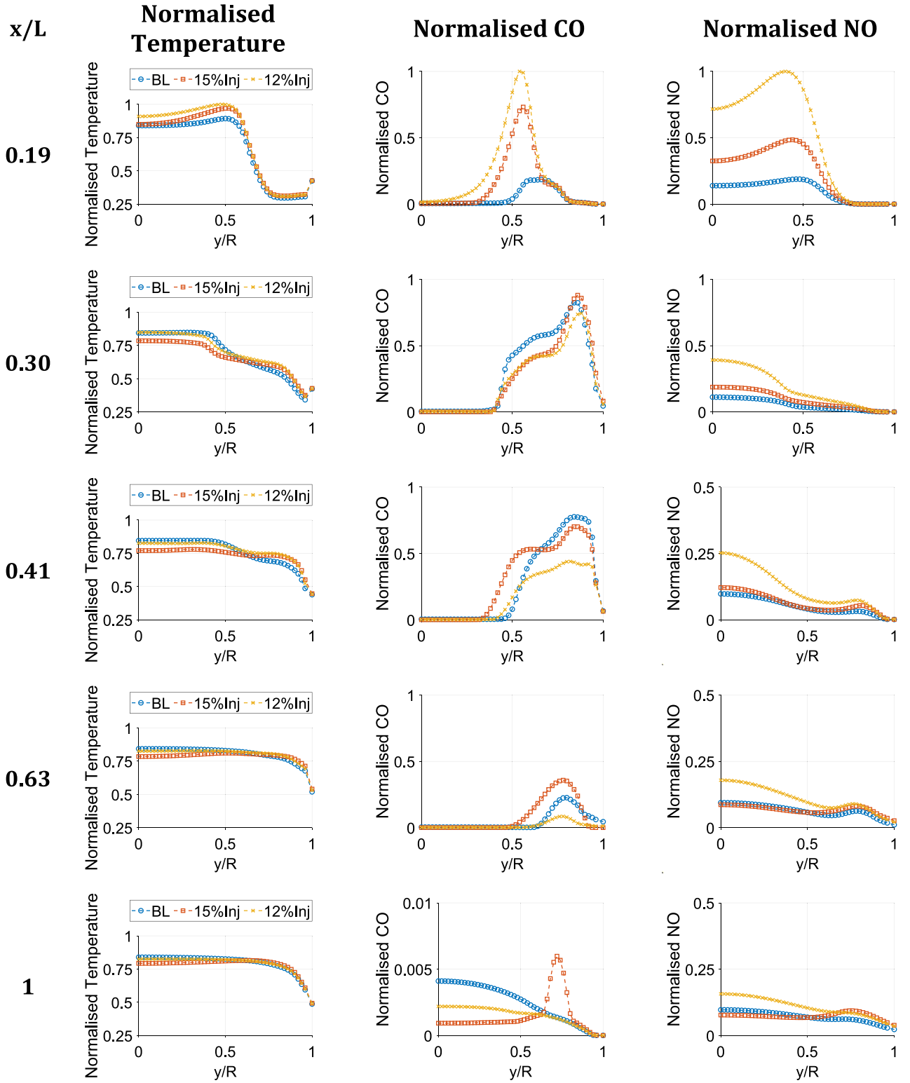
Fig. 11. Radial averaged normalised temperature, CO and NO concentrations for the baseload and injection cases at ISO across normalised axial locations.
