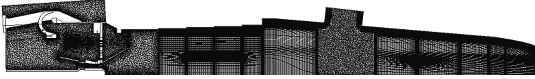
Fig. 4. Computational mesh of the quarter-model [19].
