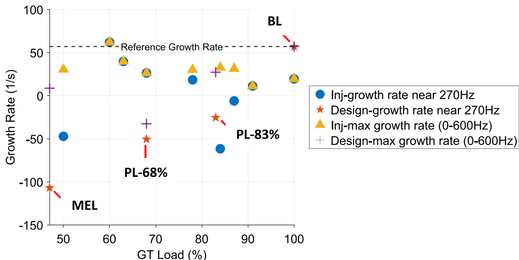
Fig. 17. Growth rates of the design operations and injection cases for RUR with the baseload growth rate line at reference frequency ( \sim 270 Hz).
