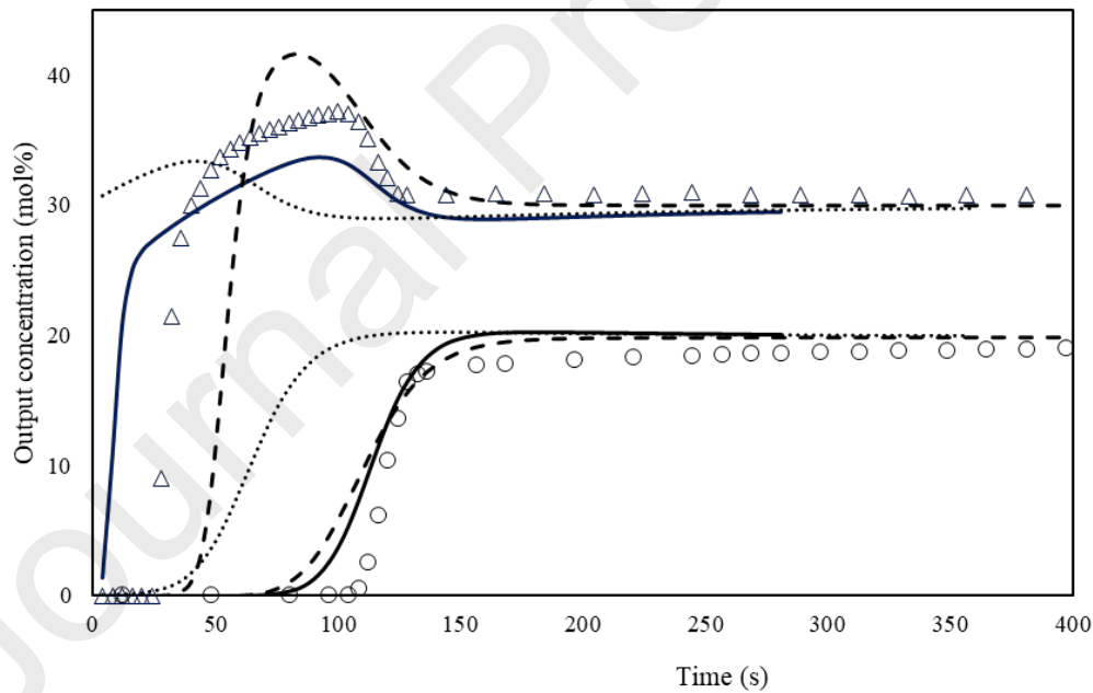
Figure 8: sensitivity analysis of MTCs at 2 bar and 0 °C. Legend: \Delta CH_4 experimental, \circ CO_2 experimental, — Case 1: MTC ( CO_2 ): 0.9/ MTC ( CH_4 ): 0.008 (1/s), - - - Case 2: MTC ( CO_2 ):0.9 / MTC ( CH_4 ):0.3 (1/s), and ..... Case 3: MTC ( CO_2 ):0.4 / MTC ( CH_4 ):0.008 (1/s)
