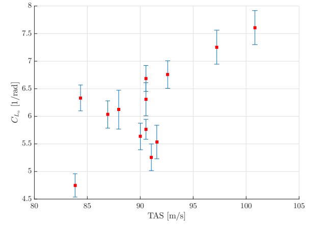
(d) Identified lift force due to \alpha
