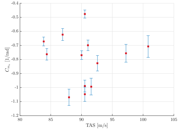
(b) Identified pitching moment due to \alpha
