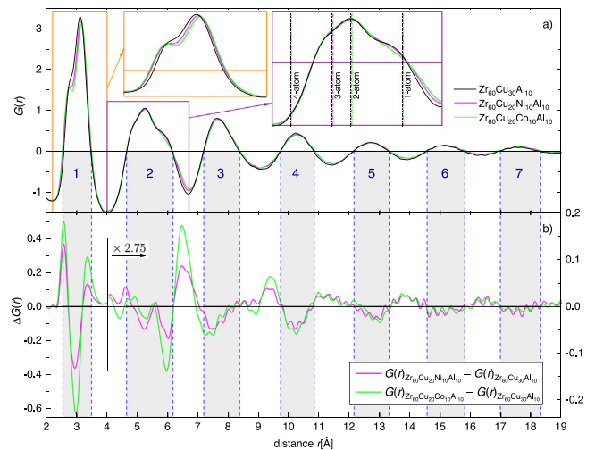
Fig. 6. a) The reduced pair distribution functions G(r) for all three alloys together with enlarged views for the first and second NN shell. The dotted vertical lines and shaded areas highlight the regions of the NN shells (as numbered). Vertical lines in the inset for the second NN shell mark expected distances if interconnected coordination polyhedra sharing 1-, 2-, 3- and 4-atoms, respectively, are assumed. b) Differences \Delta G(r) in the reduced PDF induced by alloying (the y-axis has been scaled by a factor of 2.75 from r = 4 \text{ \AA} onwards for clarity).
