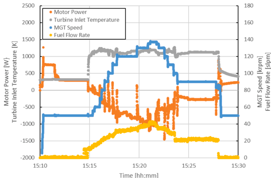
Fig. 14. MGT simple cycle test measurements for 31 March 2022.
