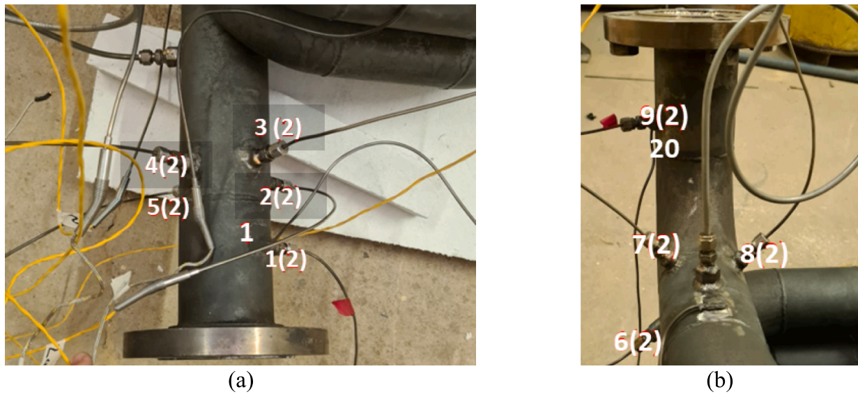
Fig. 6. Insertion thermocouple locations (a) at the receiver inlet using thermocouples '2(2)' to '5(2)' and (b) at the receiver outlet using thermocouples '6(2)' to '8(2)'.
