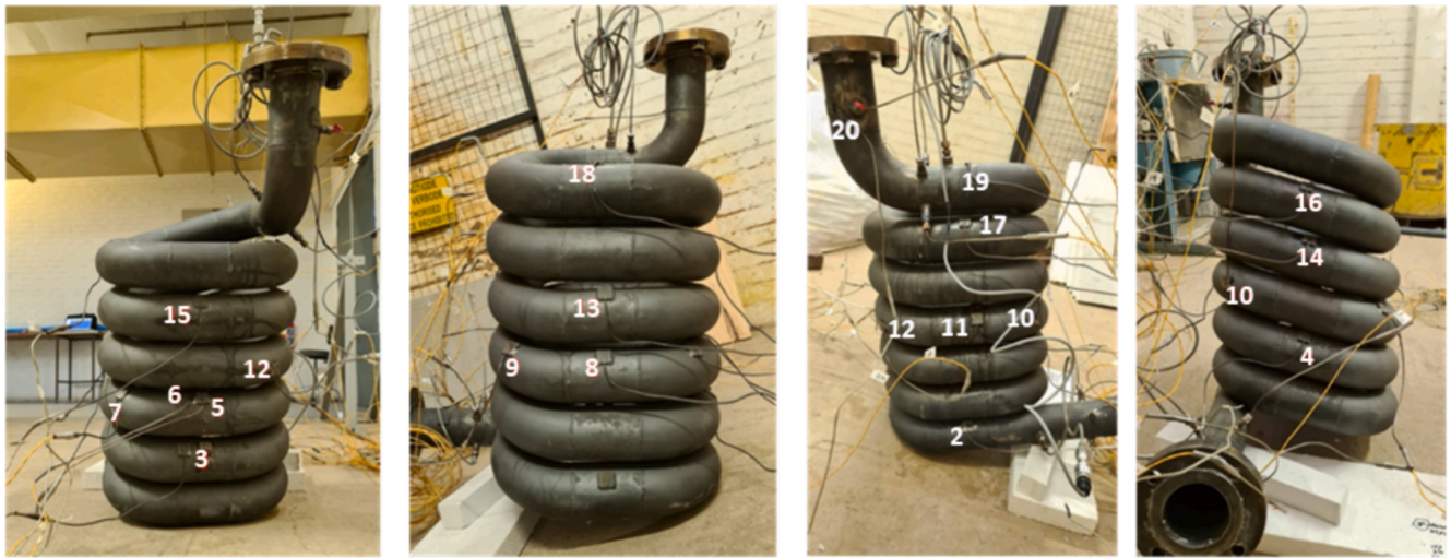
Fig. 5. Receiver coil surface-thermocouple locations (type-K).
