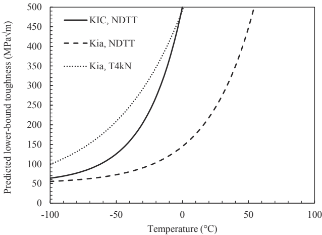
Fig. 23. Master curves for material M05.
