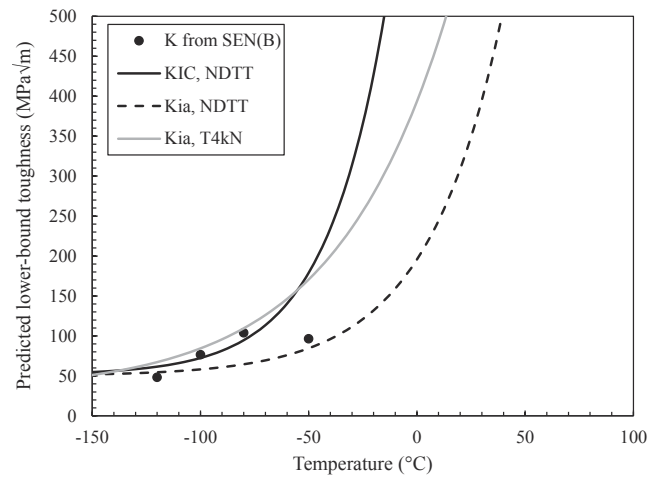
Fig. 17. Master curve predictions of toughness at a range of temperatures for M06.
