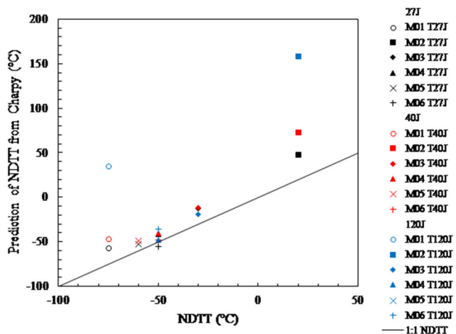
Fig. 16. Prediction of NDTT from Charpy reference temperatures.
