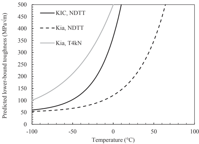
Fig. 22. Master curves for material M04.
