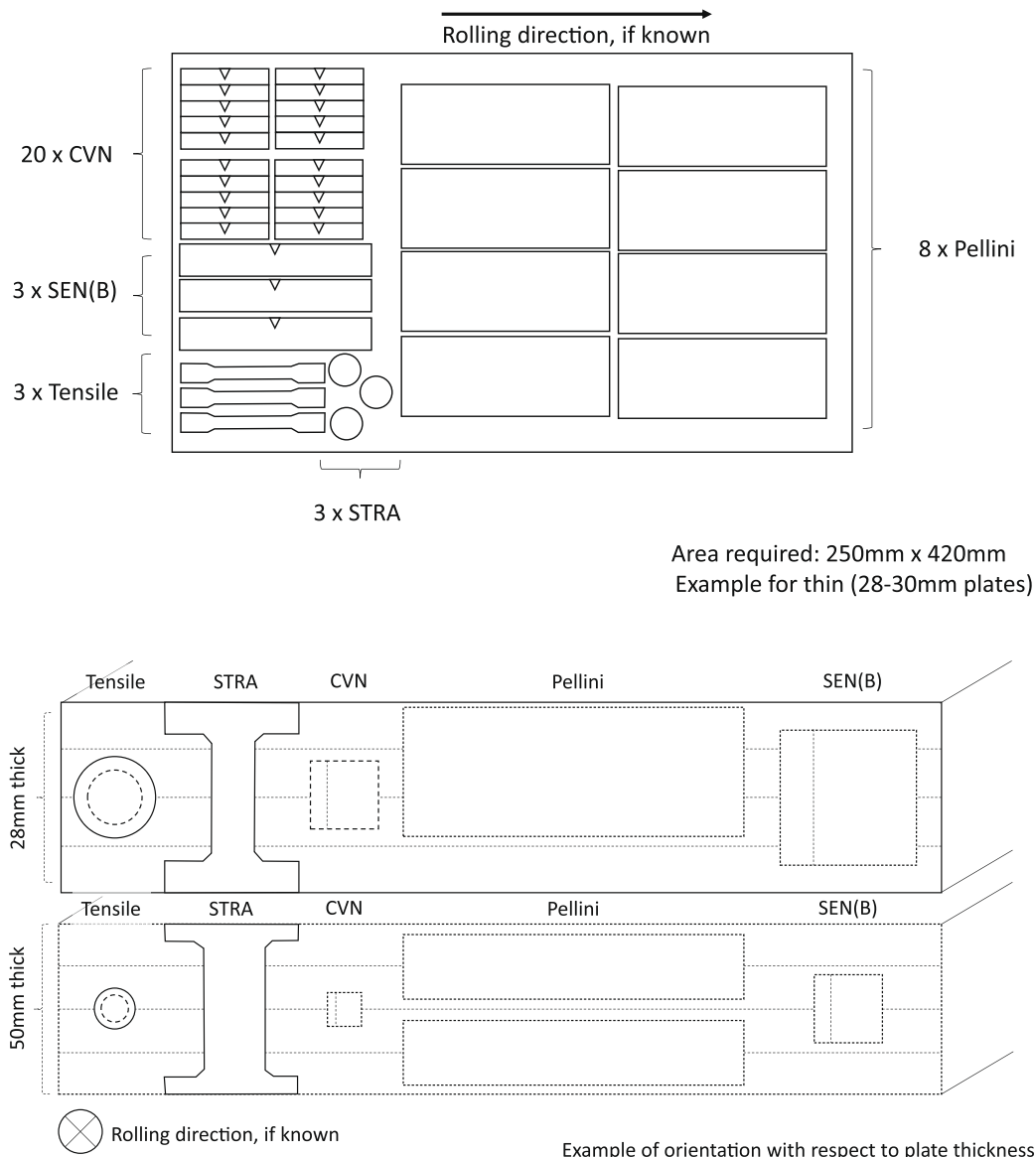
Fig. 18. Sectioning plan to show the specimen orientations with respect to rolling direction and plate thickness.
