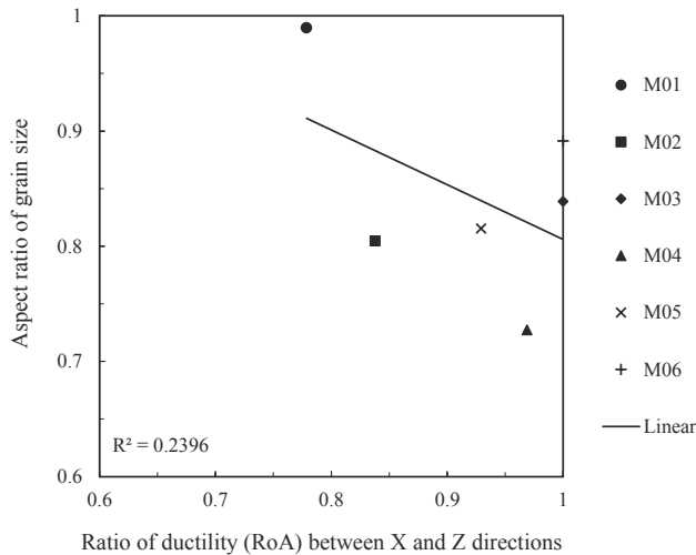
Fig. 4. Correlation between grain size aspect ratio and ratio of ductility in the rolling direction.
