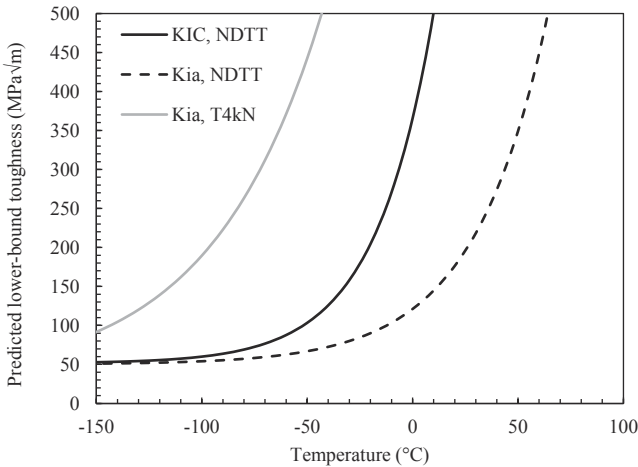
Fig. 24. Master curves for material M06.
