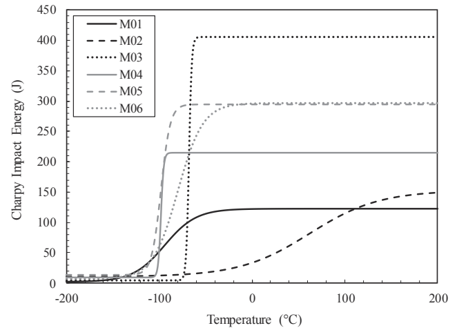
Fig. 6. Charpy curve for each material given as a tanh fit to the data.
