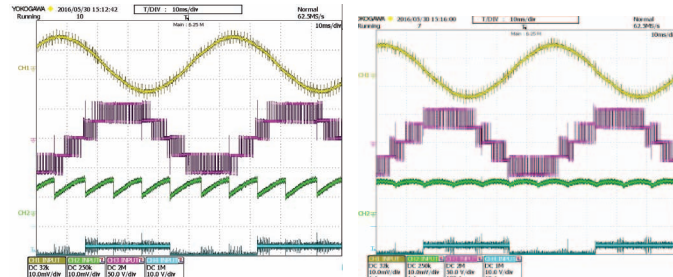
Fig. 21 Influence of phase shift “ \chi ” in switching mode II on main source current. Channel 1(yellow) motor phase A current, Channel 2(green) battery current, Channel 3 (purple) voltage between phase A and B, Channel 4(blue) 3phase bridge phase A gate signal.
