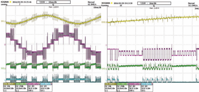
Fig. 22 Alternated switching between modulation in mode II and IV for \alpha=\pi/12 . Channel 1(yellow) motor phase A current, Channel 2(green) battery current, Channel 3 (purple) voltage between phase A and B, Channel 4(blue) 3phase bridge phase A gate signal.
