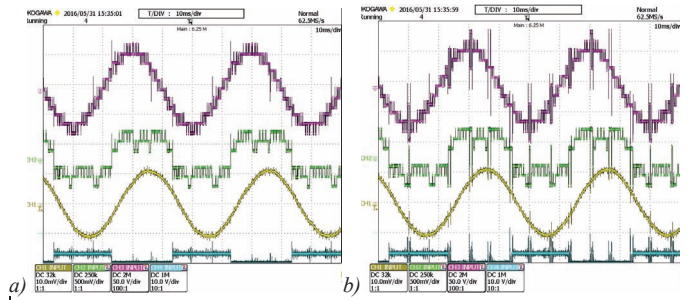
Fig. 24 Modulation of output voltage with six step switching of 3phase bridge a) mode II only, b) mode II with added mode VI. Channel 1(yellow) motor phase A current, Channel 2(green) phase A line voltage, Channel 3 (purple) voltage between phase A and B, Channel 4(blue) 3phase bridge phase A gate signal.
