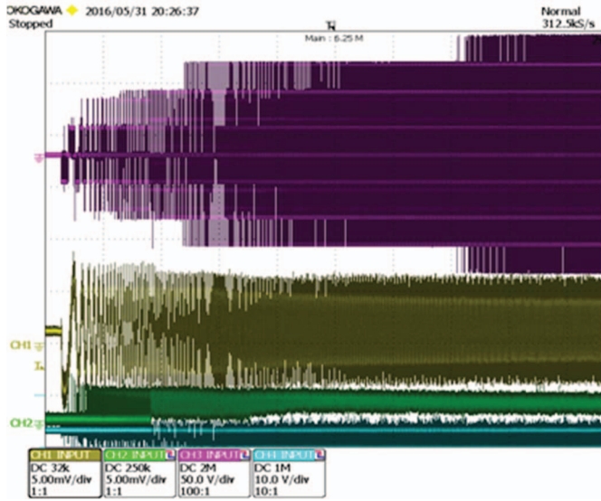
Fig. 27 Motor acceleration from 0 rpm to 200rpm with battery current limitation. Channel 1(yellow) motor phase A current; Channel 2(green) battery current; Channel 3 (purple) voltage between phase A and B; Channel 4(blue) 3phase bridge phase A gate signal.
