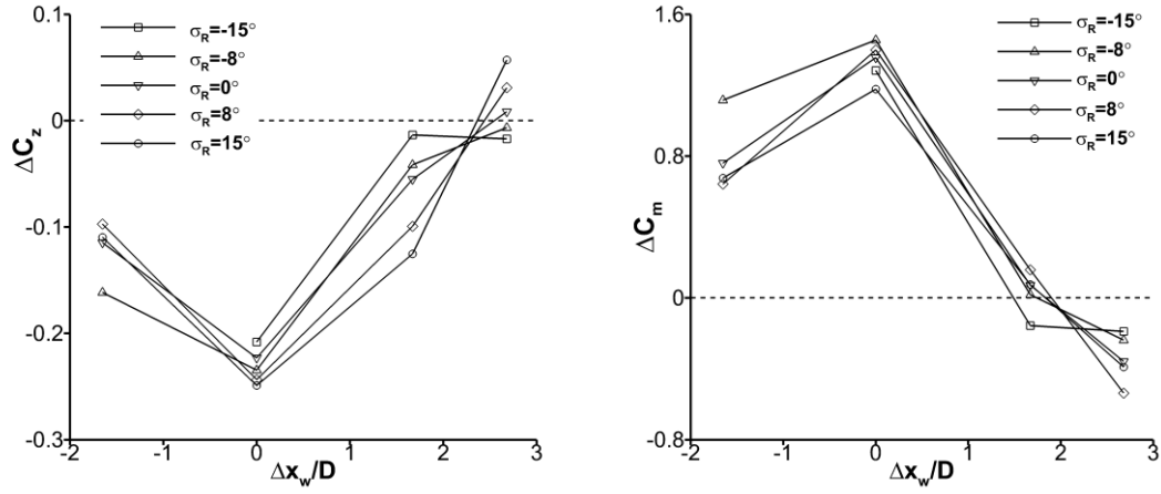
Fig. 10 Effect of axial stagger for \Delta z_w/D=2.94 , \sigma_G=0^\circ for \sigma_R=-15, -8, 0, 8, 15^\circ on (a) measured receiver normal force interference load (b) measured receiver pitching moment interference load.
