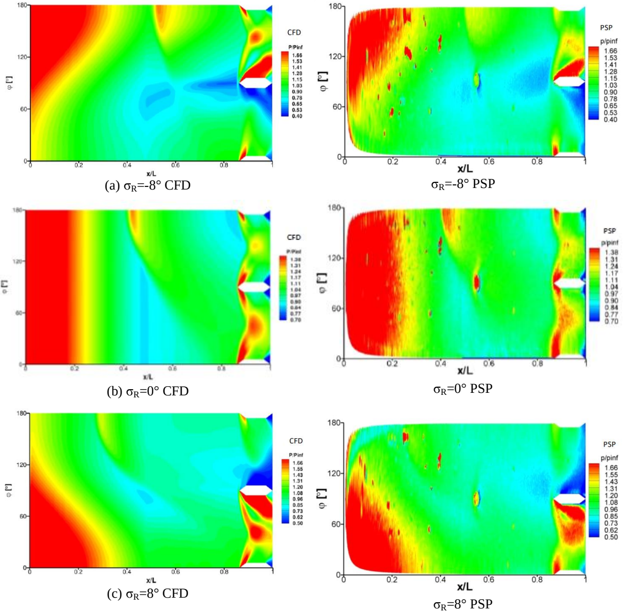
Fig. 24 Comparison of measured (PSP) and predicted (CFD) surface pressures on finned receiver for different receiver incidence settings (a-c): sharp generator, \Delta x_w/D=1.67 , \Delta z_w/D=2.94 , \sigma_G=0^\circ
