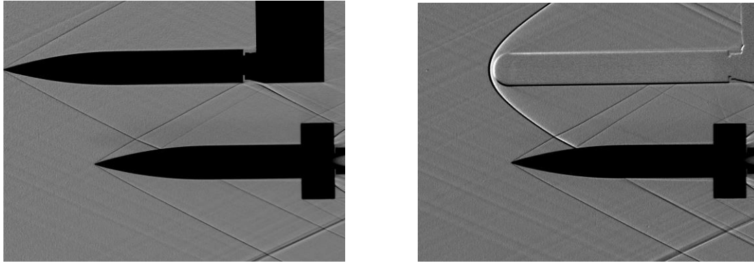
Fig. 22 Comparison of shadowgraphs for the sharp and blunt generators with \Delta z_w/D = 2.94 , \sigma_G = 0^\circ \sigma_R = 0 (a) sharp generator and receiver body: \Delta x_w/D = 2.68 (b) blunt generator and receiver body: \Delta x_w/D = 0.44 .
