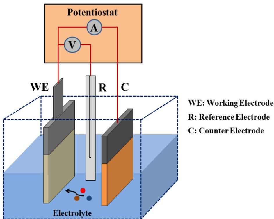
Figure 2. Schematic diagram of an electrodeposition setup [30]. Reprinted with permission from [30]; 2019 Mediterranean Journal of Chemistry.
