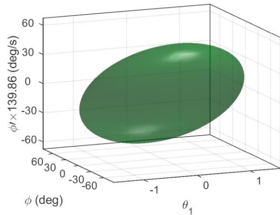
Fig. 5 ROA Estimation in the three-dimensional space
