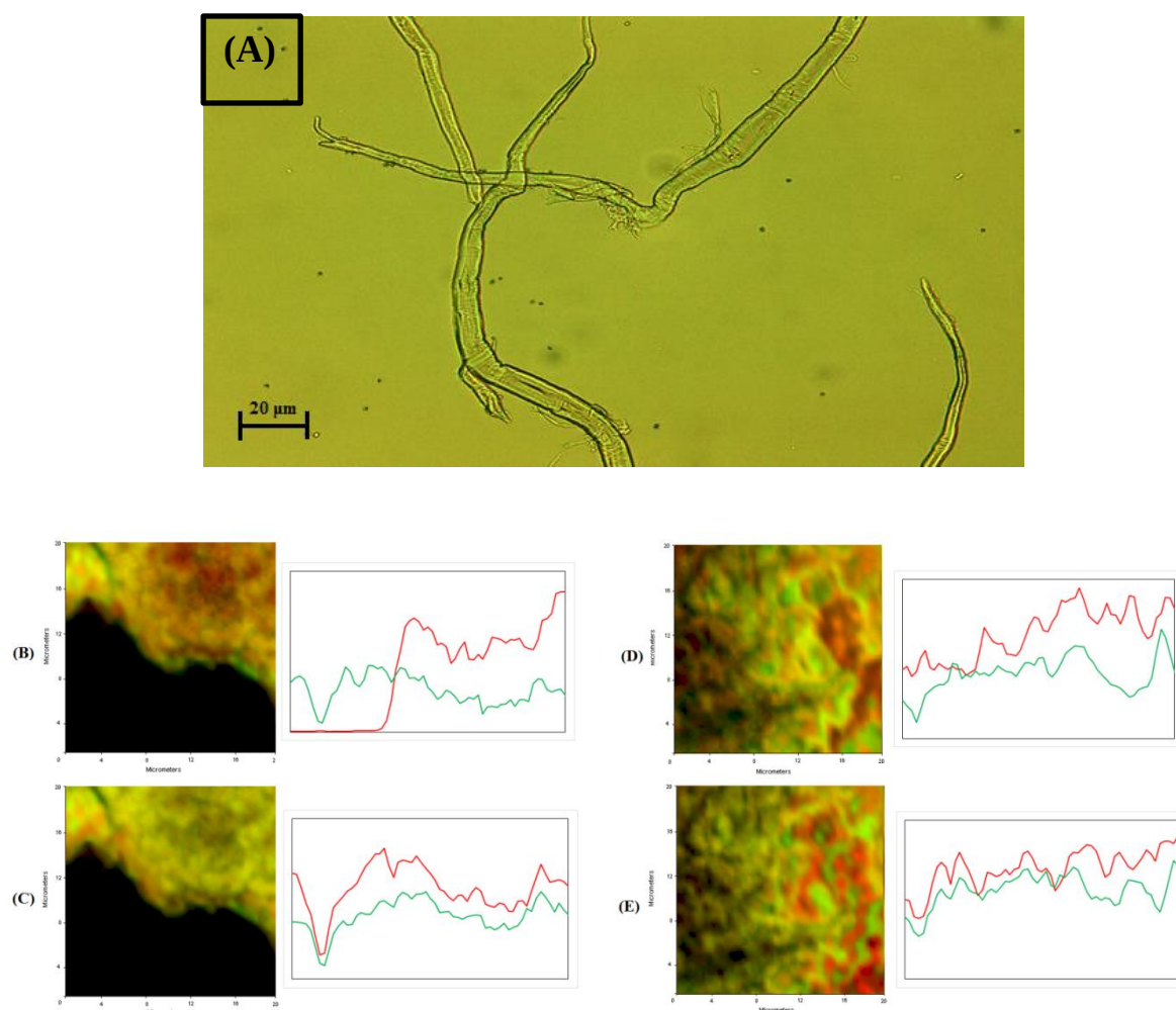
Figure 2. Image (A) - Strands from MA564 viewed under a microscope. Images (B), (C) - 20 x 20 \mu\text{m}^2 FTIR images of strand edge with the corresponding cross section spectra of the strand edge. Images (D), (E) - 20 x 20 \mu\text{m}^2 FTIR images of strand center with the corresponding cross section spectra of the center of the strand. Red regions in images (B) to (E) are the relative intensities of the protein amide I peak at 1630\text{ cm}^{-1} . Green regions in (B) and (D) are the relative intensities of the carbohydrate C-O vibration at 1030\text{ cm}^{-1} , and in (C) and (E), are the relative intensities of the acidic carbohydrate anion \text{COO}^- vibration at 1330\text{ cm}^{-1} . The regions of orange and yellow in (B) to (E) are the overlaps of the respective chemical regions in the image. For full dataset, please see supporting information Figure S3.4.
