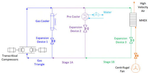
Figure 1: SCHEMATIC OF THE CRANFIELD UNIVERSITY sCO 2 RIG
