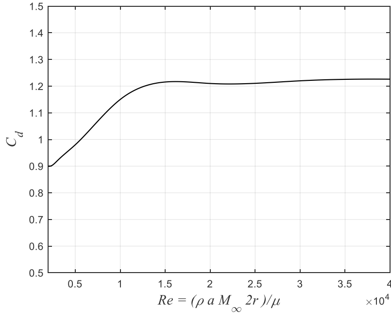
Fig. 3 Drag coefficient of a smooth, infinite-length, circular cylinder as a function of its Reynolds number in the range relevant to the current aero-whisker design (based on data from [27]).
