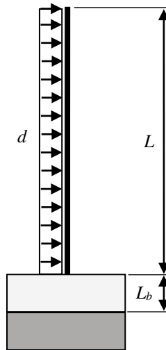
Fig. 2 Cantilever-beam model with distributed (drag) force.
