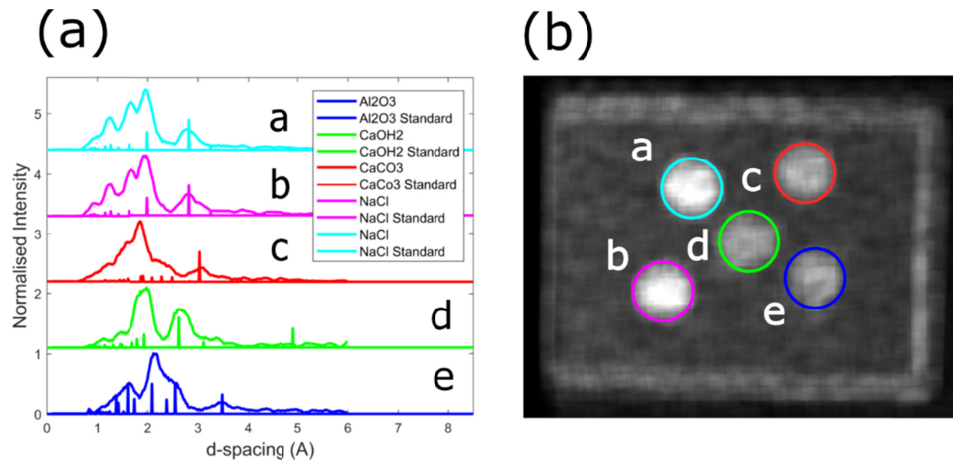
Fig. 4. (a) Conventional 1D-diffractograms for the five samples detailed in Table 1. These are generated by integrating the signals in the corresponding regions of interest as highlighted in the coherent scattering z projection (b).
