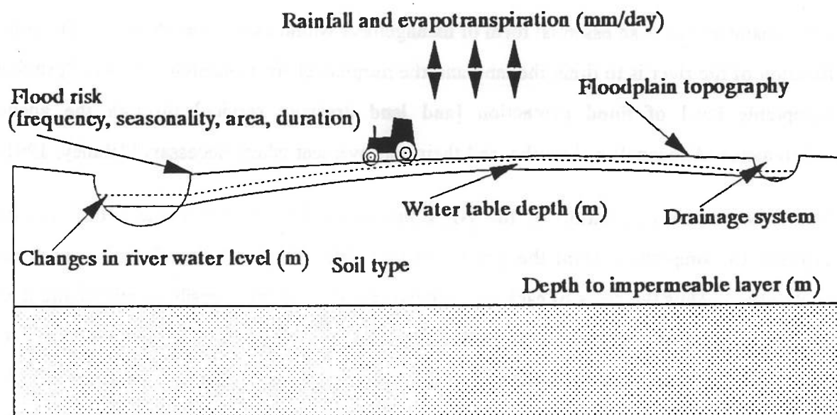
Figure 2.1 Influence of maintenance on flooding and land drainage
