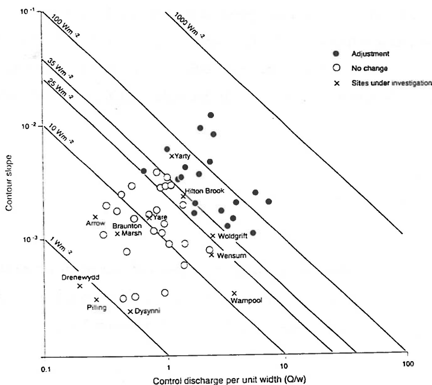
Figure 4.1 River stability (Relationship between bankfull discharge, width and slope)
