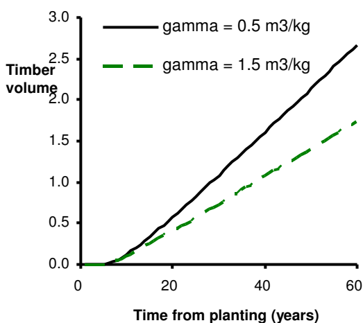
Fig. 2 Comparison of a) relative wheat yields (-) and b) tree yields ( \text{m}^3 \text{ tree}^{-1} ) at a constant k_r (0.8) and phased k_r (Eqn. 2) for wild cherry and a crop pF critical value of 2.3, c) relative crop yields and d) tree yields for two different pF critical values, e) relative crop yields and f) tree yields for two different values of \gamma .
