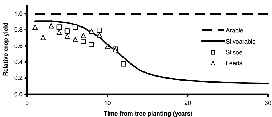
Fig 3 Validation of Yield-SAFE: model prediction of relative yield of continuous winter wheat, compared with monoculture wheat yield, in a poplar agroforestry stand ( 156 \text{ trees ha}^{-1} ), compared to observed relative crop yields in Silsoe and Leeds agroforestry experiments, 1992-2004 (open symbols).
