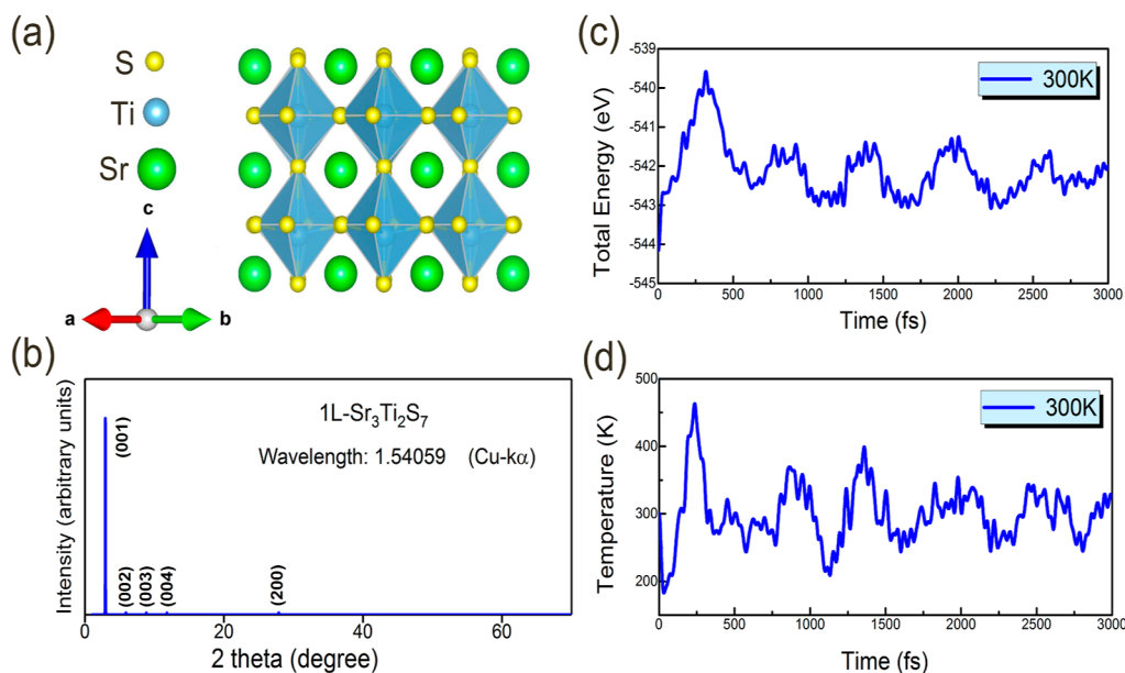
Figure 1. Lattice structure, X-ray diffraction (XRD), and structural stability of two-dimensional Sr 3 Ti 2 S 7 perovskite. (a) Perspective view of the natural super lattice nanostructure in Sr 3 Ti 2 S 7 perovskite. The green and yellow spheres represent the Sr and S atoms, respectively. The TiS 6 octahedra are in blue. (b) The XRD patterns for two-dimensional Sr 3 Ti 2 S 7 perovskite with the wavelength of 1.54059 Å (Cu Kα) calculated by using the VESTA package (3D visualization program for structural models, volumetric data such as electron/nuclear densities, and crystal morphologies) and bulk Sr 3 Ti 2 S 7 perovskite are shown in Figure S2 of the Supporting Information. (c,d) The ab initio molecular dynamics on total energy and temperature at 300 K.
