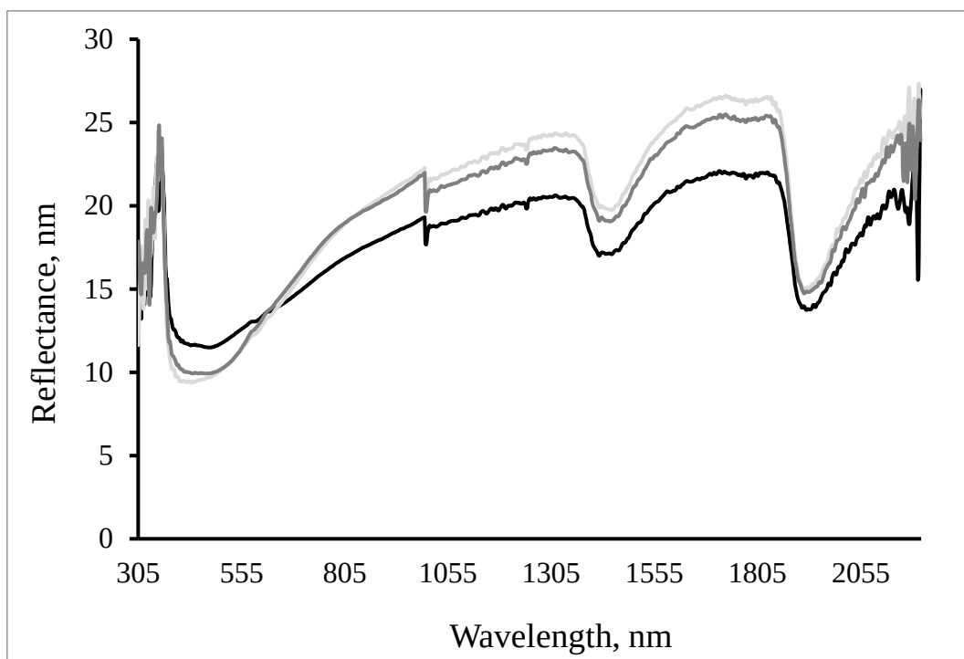
Figure 2. Examples of the raw on-line soil visible and near infrared (vis-NIR) spectra, collected with the on-line sensor. Showing slight deviations in relative absorbance, across the wavelengths, which is dependent on the soil properties.
